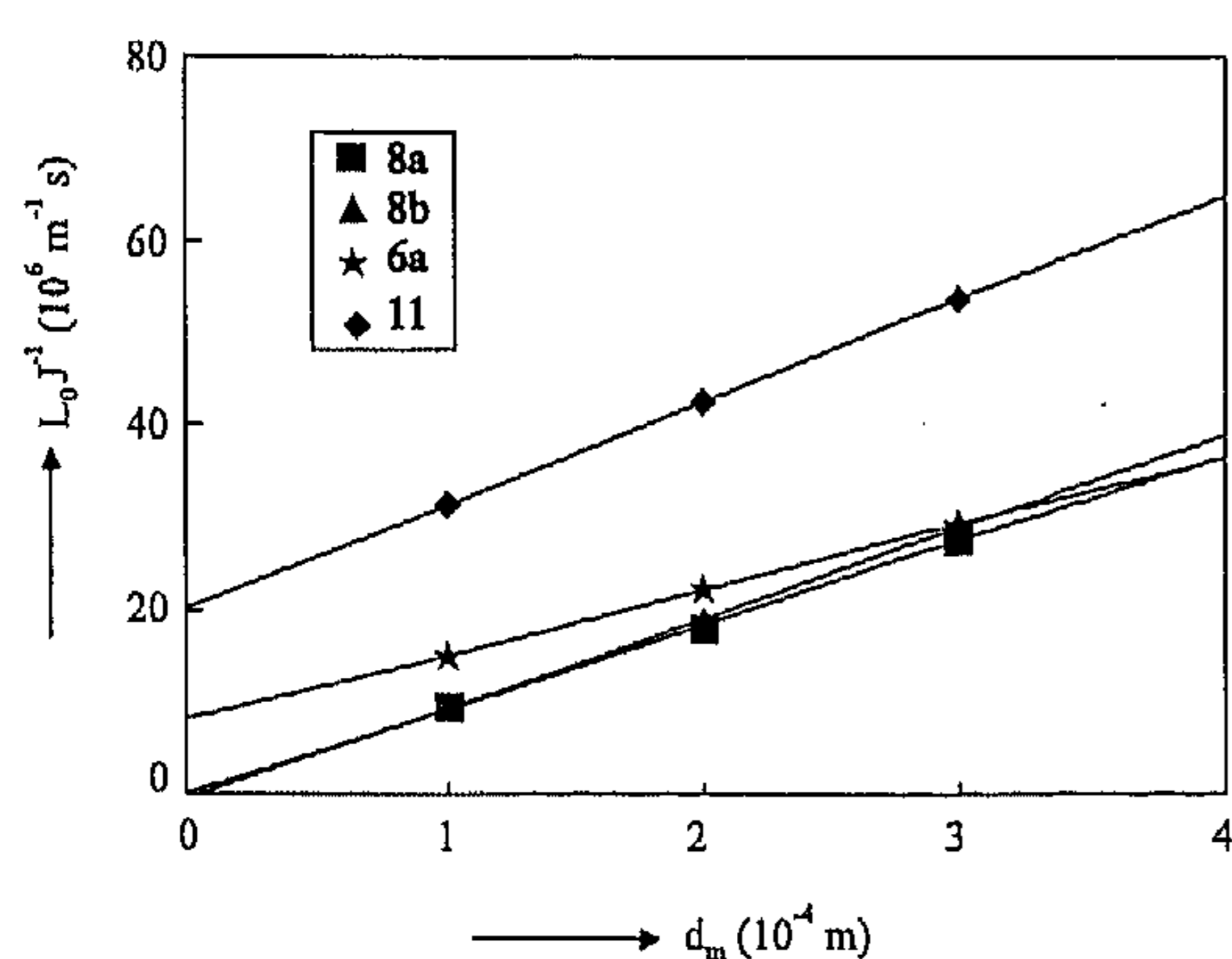
Fig. 5. Influence of the membrane thickness ( n \times 100 \mu m ) on L_0/J (See Eq. (2): L_0/J = (1 + \alpha)D_m^{-1}d_m ) [28]; [carrier]_m = 1 \times 10^{-2} M , source phase: 1 \times 10^{-1} M KClO_4 , T = 298 K.
