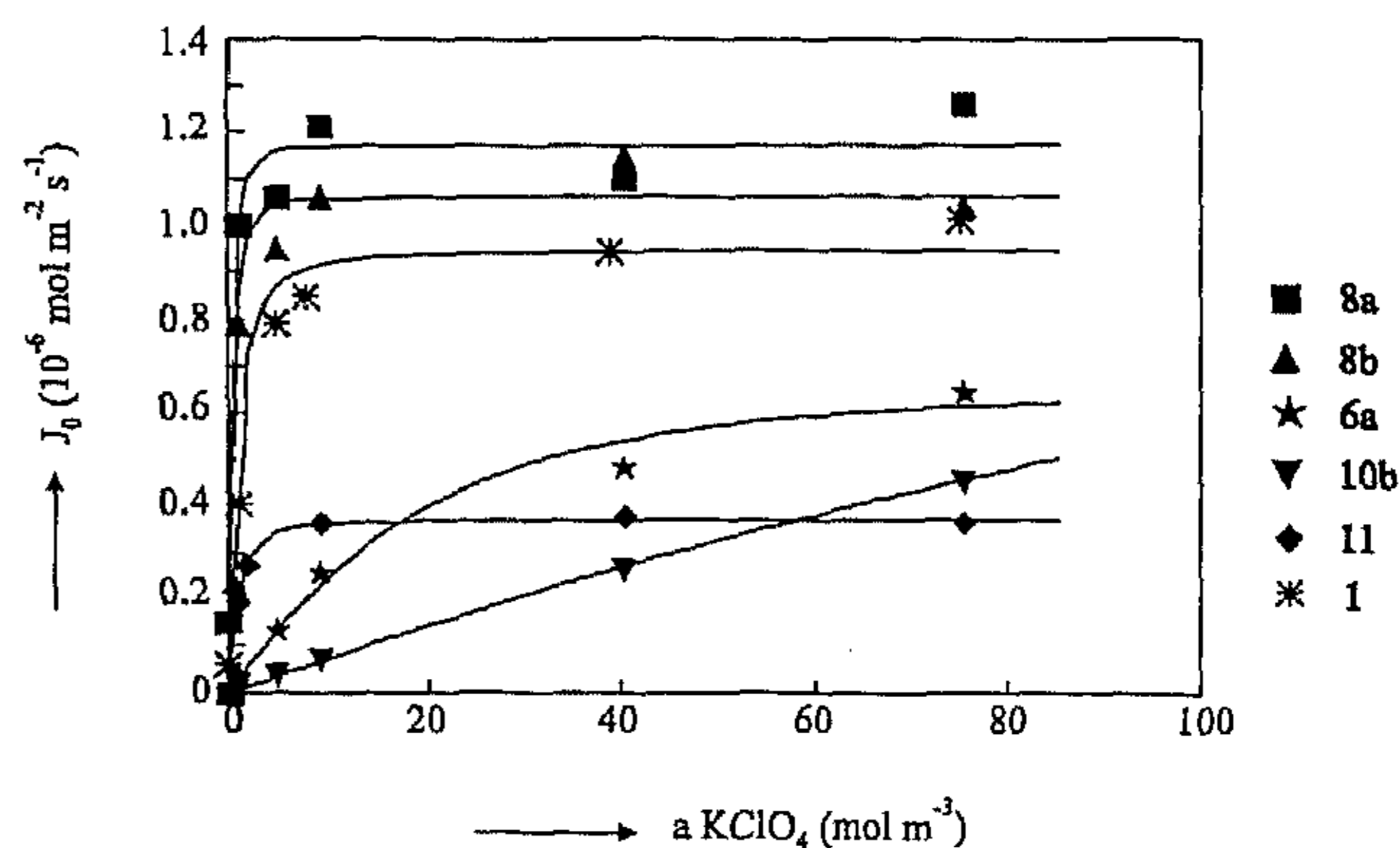
Fig. 4. \text{KClO}_4 flux as a function of the salt activity a in the source phase ( [\text{carrier}]_m = 1 \times 10^{-2} \text{ M} ; T = 298 \text{ K} ). The lines drawn are calculated with the model; the points are measured values.
