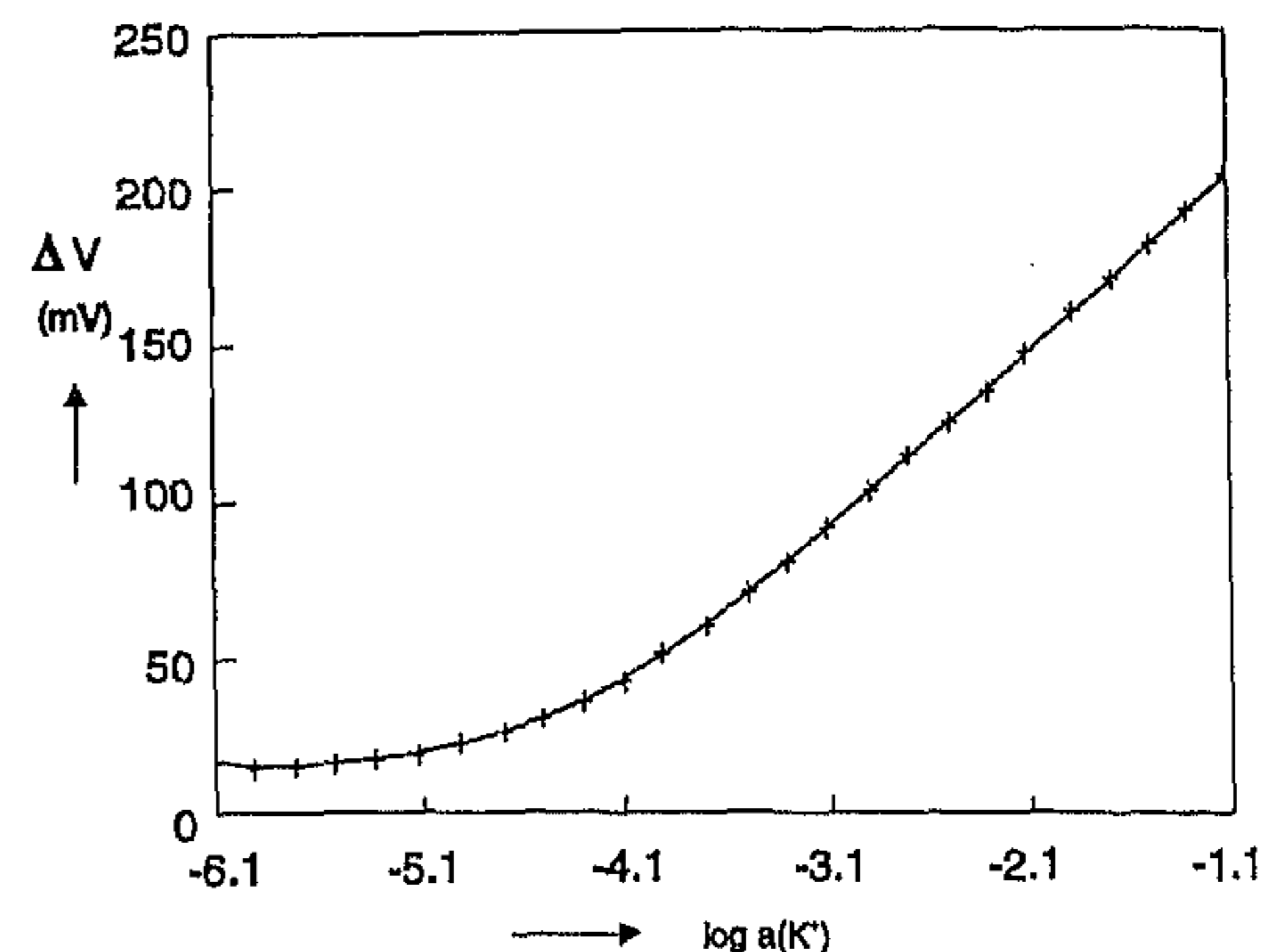
Fig. 8. \text{K}^+ response of CHEMFETs containing ionophore 8a in the presence of 1 M \text{NaCl} .
