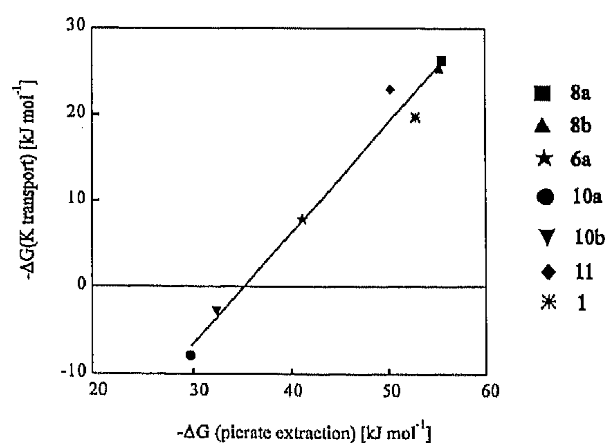
Fig. 7. Linear free energy relationship between \Delta G_{ox} obtained from membrane transport through NPOE, and the association constant of K-picrates in CHCl_3 .
