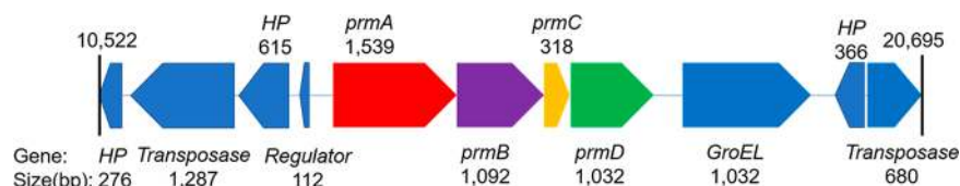
Figure 1. Scheme of the propane monoxygenase ( prmABCD ) gene cluster. The numbers on the above left and right sides indicate their locations in Plasmid_3. The arrows indicate genes, and the strings between them indicate the gaps between different genes. The lengths of the strings and the arrows are proportional to their relative sizes. The right or left direction of the arrows indicates a positive or negative strand. Gene name abbreviation: HP (hypothetical protein), Regulator (two-component system response regulator), prmA (propane monoxygenase alpha subunit), prmB (propane monoxygenase beta subunit), prmC (propane monoxygenase coupling protein), prmD (propane monoxygenase reductase protein), and GroEL (chaperonin GroEL ).
