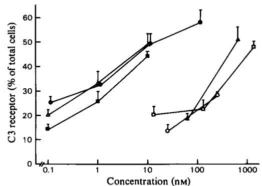
Fig. 3. Comparison of the effects of various derivatives of cholecalciferol on the formation of C3 receptors of HL-60 cells
