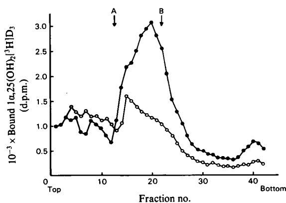
Fig. 7. Sucrose-density-gradient analysis of 1\alpha,25(\text{OH})_2[^3\text{H}]\text{D}_3 binding by cytosol preparations. Cytosol protein (approx. 5 mg) was incubated with 10\text{ nM} 1\alpha,25(\text{OH})_2[^3\text{H}]\text{D}_3 (●) or the same concentration of 1\alpha,25(\text{OH})_2[^3\text{H}]\text{D}_3 plus a 1000-fold excess of 1\alpha,25(\text{OH})_2\text{D}_3 (○) and analysed on 4–20% sucrose gradients. Arrow A indicates the elution position of chymotrypsinogen (2.5 S) and arrow B shows that of bovine serum albumin (4.4 S).
