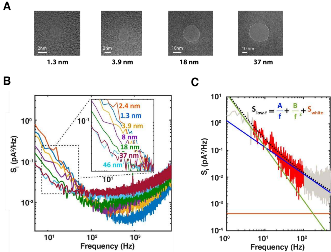
Figure 2. (A) TEM micrographs of the measured pores. Diameters were calculated from conductance measurements using Eq.S3. (B) Current power spectral density of nanopores with different diameters between 1.3 and 46 nm. The inset shows a zoom-in of the low frequency regions. (C) Example fit of the low-frequency ionic current power spectral density for a 2.4 nm pore. Dotted black line is the fit to the data (red) as reported by Equation (19), which comprises 1/f (blue), Lorentzian (green) and white noise (orange) contributions. The rest of the spectrum, out of the fitted region, is shown in light grey. Extracted values of A , B , and the calculated S_{white} are reported in Table (S1).
