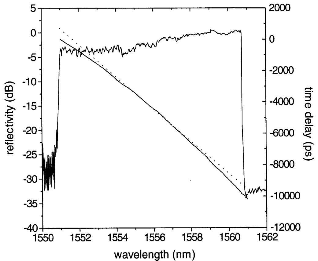
Fig 2. Reflectivity and time delay of a 1\text{m} \times 10\text{nm} grating designed to compensate for 2^{\text{nd}} and 3^{\text{rd}} order dispersion of 578 km of AT&T TrueWave fibre. The dotted line shows the theoretical linear time delay of -1.67\text{ ps/nm}\cdot\text{km} for a 578 km link of this fibre.
