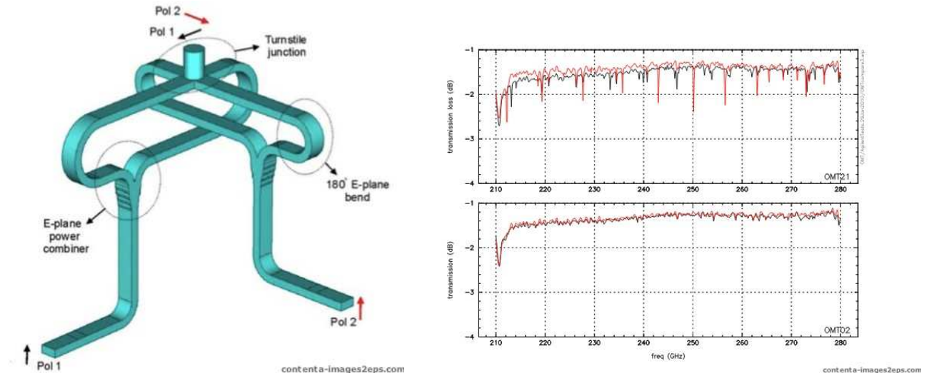
Figure 4: Left: a diagram of the waveguides inside the OMT. Right: passbands for a poorly behaved OMT with resonances (top) and a well behaved OMT without them (bottom).
