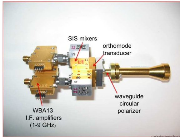
Figure 1: Left: a 1 mm dual-polarization receiver.
