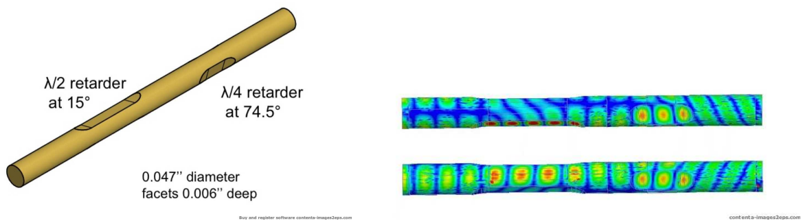
Figure 2: Left: the mandrel, which was used as a mold for the inside of the polarizer; the two flats are separated by an angle of 59.5^\circ , and act as a wideband circular-to-linear converter. Right: the HFSS simulation showing radiation being converted from circular to linear polarization as it propagates from right to left.
