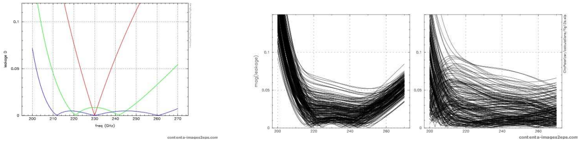
Figure 3: Left: the theoretical leakage percentage as a function of frequency using polarizers with one (red), two (green), and three (blue) sets of flats. Center: leakages for the two-section polarizer, simulated using machining errors of 0.0003" in the depth of the flats and 0.2° errors in the angle between the flats. Right: leakages for the three-section polarizer using the aforementioned machining errors.
