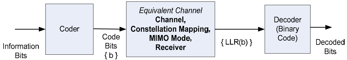
5 6 Figure 9: Bit Interleaved coded modulation system
