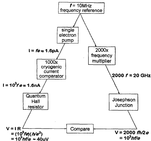
Fig. 8. Block diagram of the metrology triangle experiment.
