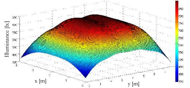
Fig.3: The distribution of horizontal illuminance at the CF, Min.336 lx and Max.894 lx.
