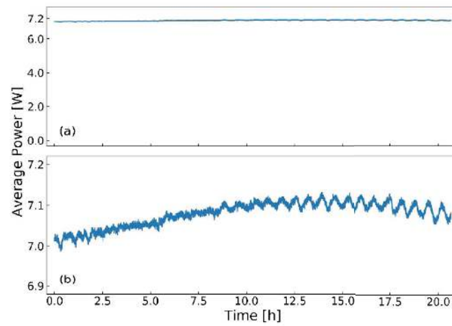
Fig. 6. (a) Laser output power over a period of 20 h. A slight long-term variation of less than 1% of the 7.05 W average power is observed. (b) shows a zoomed view of (a).
