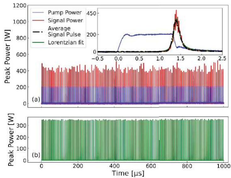
Fig. 3. (a) Typical pulse train at 11.2 W output power and 140 kHz repetition rate. The inset shows an example of timing synchronization of the pump and signal pulses, as well as a signal pulse averaged over 60 samples. The signal peak power is evaluated at 420 \pm 70 W. (b) Lorentzian fit for each pulse shows the average gain-switched envelope. The average peak power is 345 W with an RMS variation of 3 W.
