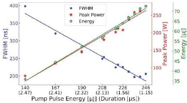
Fig. 5. Energy, duration, and peak power of the signal pulses as a function of the pump pulse energy and duration, for a fixed repetition rate of 100 kHz. For each point, the pump peak power and duration are adjusted to prevent the onset of a secondary pulse per cycle.
