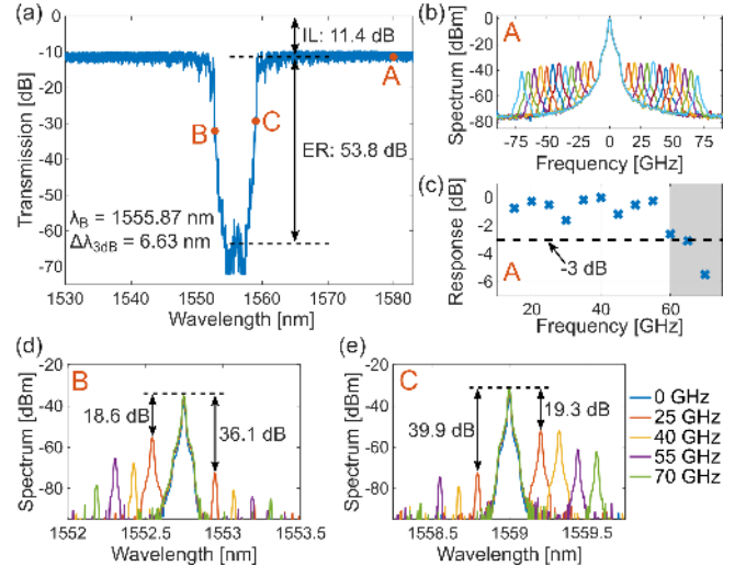
Fig. 2. (a) Optical transmission of the WBG modulator. (b) Optical modulation spectra for a sinusoidal microwave signal at frequencies between 15 GHz and 70 GHz. The optical carrier wavelength is 1580 nm. (c) The 3 dB bandwidth of the RF response of the on-chip electrodes is estimated to be around 60 GHz. (d), (e) Asymmetric optical modulation spectra for different microwave frequencies with the optical carrier at 1552.75 nm (d) (point B in (a)) and at 1559 nm (e) [point C in (a)].
