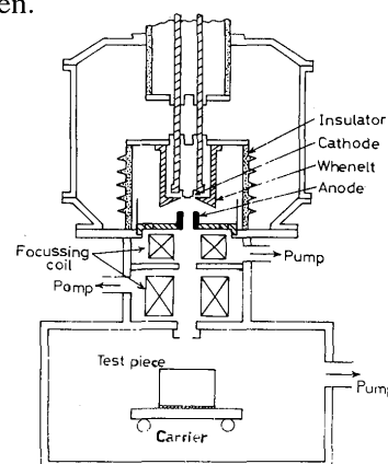
Fig. 1. Schematic diagram of EB-welder.
