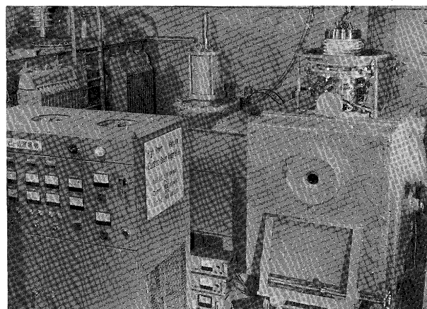
Photo 1. General view of 100 KW-EB welder which was developed by authors.
