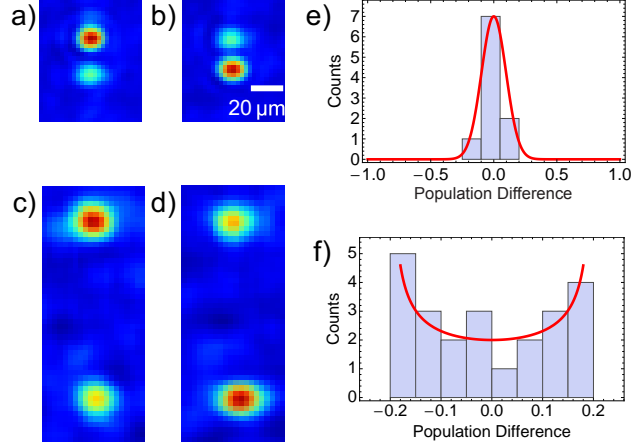
FIG. 3: (color online) a)–d) Examples of typical data showing images of the two interferometer output ports. a) and b) correspond to an interferometer with 30\hbar k SB-LMT beam splitters, while c) and d) correspond to an interferometer with 102\hbar k SB-LMT beam splitters. The fact that the atom clouds for the 102\hbar k interferometer are slightly larger than the clouds for the 30\hbar k interferometer is due to the fact that the detection time was later for the 102\hbar k interferometer than for the 30\hbar k interferometer (respectively 21 ms and 12 ms after the production of the cold cloud, so that in each case the atoms would return to our imaging region at the time of detection), which gives the clouds more time to thermally expand. e) Histogram of population difference of single \pi/2 -pulse and a normal distribution with 5% diffraction efficiency variation (standard deviation). f) Histogram of population difference of a 102\hbar k interferometer, and a synthesized distribution of an interferometer output with 18% contrast and randomly varying phase from shot to shot (red curve). The 30\hbar k interferometer output has a similar distribution with 70% contrast.
