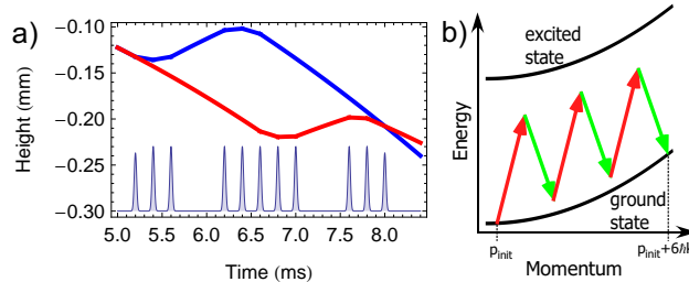
FIG. 1: (color online) a) Depiction of a sample pulse sequence and the corresponding trajectories of the interfering wavepackets. The thick lines illustrate the wavepacket trajectories, while the thin line in the bottom portion of the figure represents the temporal intensity profile of the pulse sequence. This particular sequence has SB-LMT beam splitters consisting of three 6\hbar k pulses, corresponding to a total momentum splitting of 18\hbar k . The first and final pulses of the sequence are \pi/2 -pulses, and the middle nine pulses are \pi -pulses. Each pulse has a Gaussian temporal profile. b) The energy-momentum diagram of 6\hbar k Bragg transition driven by two counter-propagating beams (green and red).
