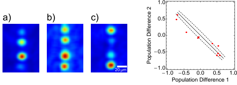
FIG. 4: (color online) Parametric plot of simultaneous 30\hbar k interferometer outputs. The upper interferometer output is plotted on the x-axis while the lower interferometer is plotted on the y-axis. The off-diagonal line shows the expected correlation between two simultaneous interferometers having phase difference \pi with 70% contrast, and the dashed curves show the atom shot noise (there are 250 atoms per interferometer at the time of detection). a)–c) Typical images at various relative phases. The lower spots correspond to the two output ports of the lower interferometer, while the upper spots correspond to the two output ports of the upper interferometer.
