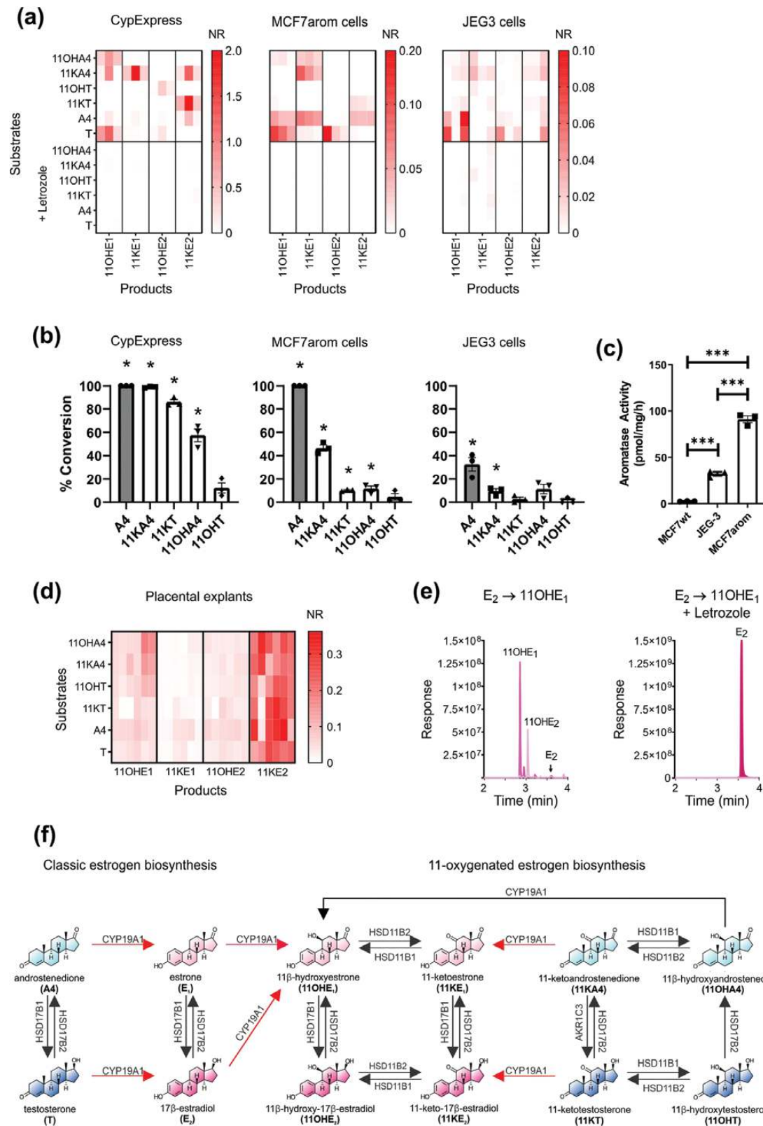
Figure 1. Biosynthesis of 11-oxygenated estrogens from 11-oxygenated and classic androgens. A, Biosynthesis of 11-oxygenated estrogens by 3 in vitro aromatase expression systems. Assays (n = 3) were performed using 1- \mu M androgen substrate with and without 10- \mu M letrozole. Owing to the lack of commercially available 11-oxygenated estrogen standards, conversion data are expressed as the mean normalized responses (NR) from independent experiments each performed in triplicate (NR: [peak area/peak area of the internal standard]/protein). B, Percentage conversion of aromatase substrates as calculated substrate utilization. Data points are shown as mean \pm SEM from 3 independent experiments each performed in triplicate. Statistical analysis was performed by comparing each steroid to its substrate specific control. *P less than .05; unpaired t test. C, Aromatase
