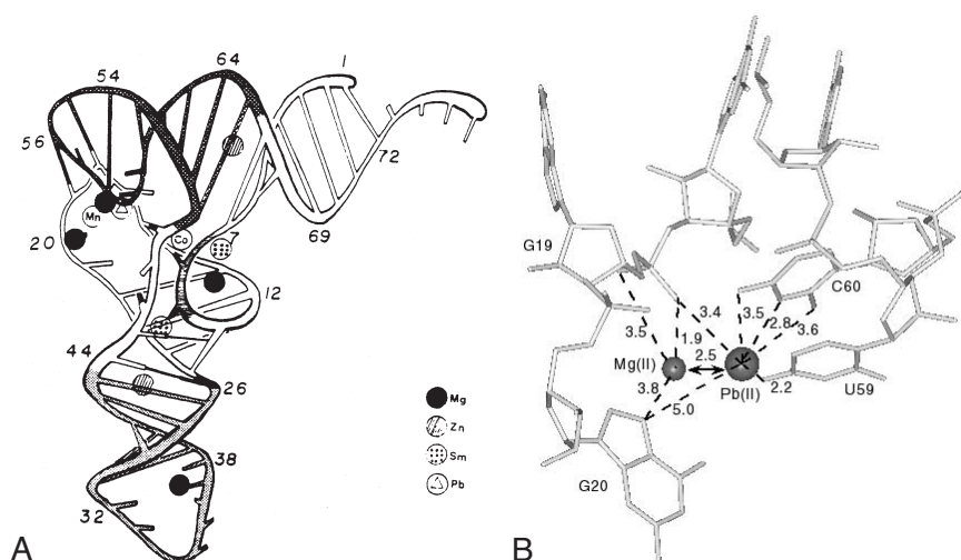
Figure 1 (A) Metal ions found in the crystal structure of yeast tRNA Phe and the relationship between these sites and the overall structure. (Reprinted, with permission, from Pan et al. 1993.) (B) Superposition of the Pb(II) and Mg(II) binding sites from the intersection of the D and TΨC loops. Waters of hydration are not shown and contact distances are given in angstroms.
