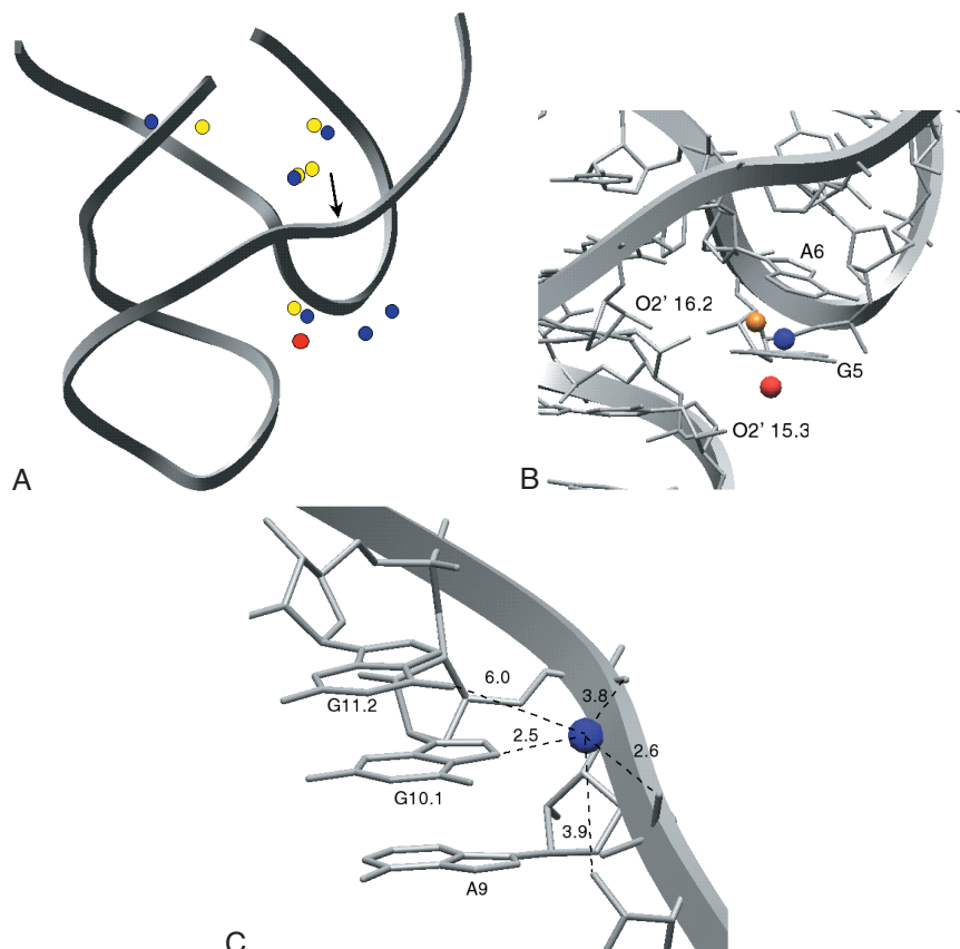
Figure 2 (A) Metal ions found in the crystal structures of the hammerhead ribozyme and the relationship between these sites and the overall structure. The location of the cleavage site is marked by the arrow. Mg(II) is shown in yellow , Mn(II) is shown in blue , and Tb(III) is shown in red . (B) Expanded view of the G5 metal-binding site of the hammerhead ribozyme. Waters of hydration have been omitted. (C) Expanded view of Mn(II) binding to the p9 site of the hammerhead ribozyme. Waters of hydration are not shown and distances are given in angstroms.
