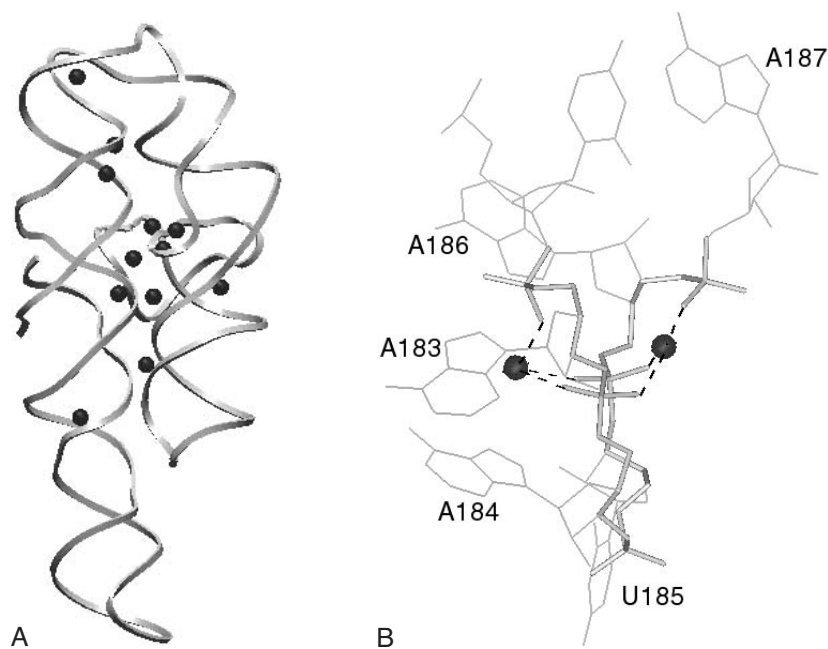
Figure 3 (A) Ribbon diagram of the P4-P6 domain of the group I intron from Tetrahymena showing the location of the bound Mg(II) ions. (B) Expanded view of the dimagnesium site from the A-rich bulge of the P4-P6 domain. The Mg(II) ions hold the backbone in a highly distorted conformation by coordination to the phosphate oxygens of A184 and A186. Phosphate oxygens from A183 and A187 also make inner sphere contacts with the Mg(II) ions. The Mg–Mg distance is 5.3 Å. The Mg(II)–O P distances range from 2.0 to 2.3 Å. Waters of hydration are not shown.
