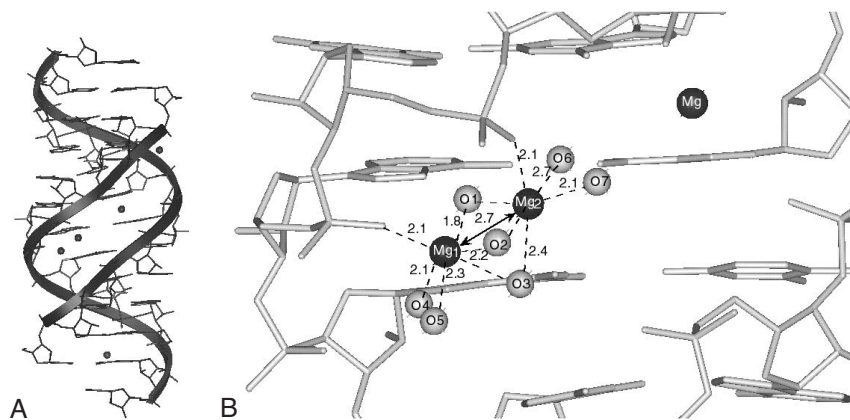
Figure 4 (A) Metal-binding sites from the loop E fragment of the E. coli 5S rRNA. (B) Expanded view of the dimagnesium center from the 5S rRNA determined at 1.5 Å resolution. Water molecules directly coordinated to the Mg ions of the dinuclear center are shown, but others have been omitted for clarity. Contact and bond distances are given in angstroms.
