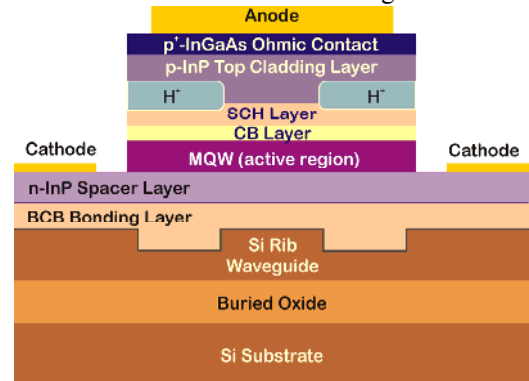
Fig. 1 Cross-section of an evanescent, hybrid III-V/Si laser based on DVS-BCB bonding.
