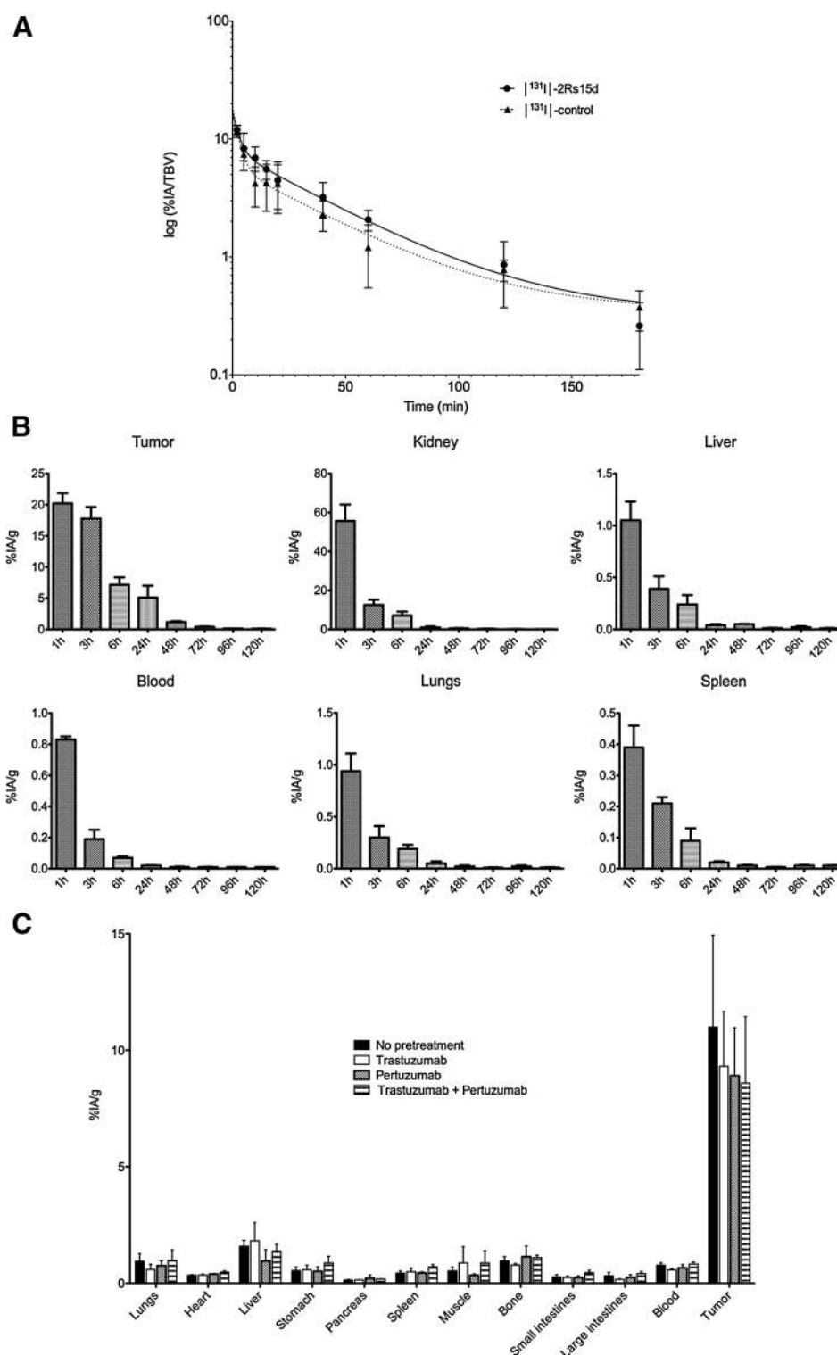
Figure 4. A, Semi-log plot of blood clearance data for [ 131 I]-2Rs15d and [ 131 I]-control sdAb in normal mice ( n = 6). Data are presented as % IA per total blood volume (% IA/TBV). B, Tumor and tissue distribution of [ 131 I]-2Rs15d in mice with BT474/M1 xenografts up to 120 hours postinjection. Data are presented as mean ± SD ( n = 3). C, Ex vivo biodistribution of [ 131 I]-2Rs15d after 1 hour in BT474/M1 tumor xenografted mice pretreated 72 hours earlier with a 100-fold molar excess of trastuzumab, pertuzumab, or both. ( n = 4). Values (mean ± SD) are expressed as % IA/g, except for thyroid for which % IA was used. No significant differences in tumor targeting were observed ( P = 0.617), determined with one-way ANOVA.
