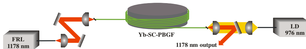
Fig. 5. Ytterbium-doped solid-core photonic bandgap fiber amplifier, seeded by an 1178 nm fiber Raman laser, and backward-pumped by a 976 nm laser diode.
