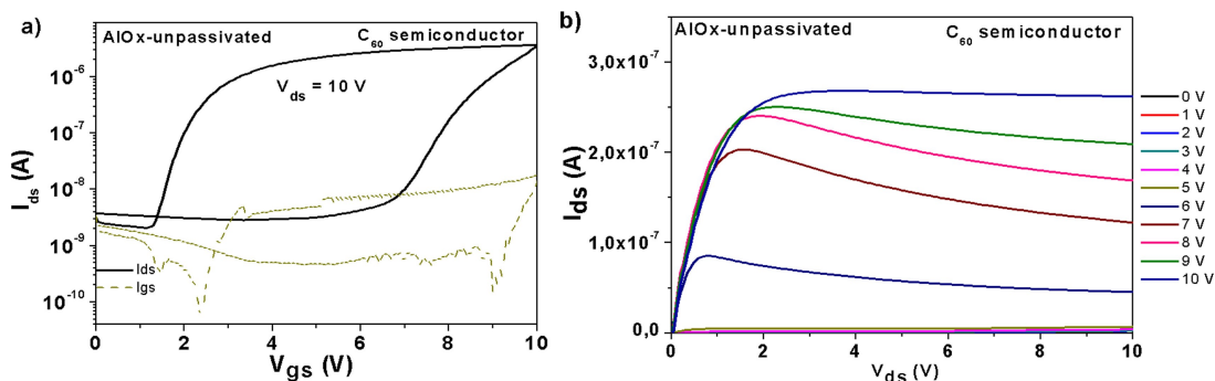
Figure 6. Unpassivated AlOx + C 60 semiconductor. a) transfer characteristics; b) output characteristics. The specific capacitance of the dielectric layer was C od = 468.6 nF/cm 2 and the electron field effect mobility \mu_e = 1.2 \times 10^{-2} cm 2 /Vs.
