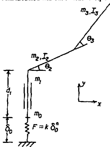
Fig. 1 Planar Manipulator on a Vertically Compliant Base
