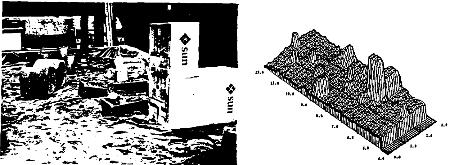
Figure 4: Obstacle course
