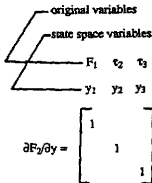
Fig. 9 \partial F_2/\partial y for a Planar Manipulator on a Vertically Compliant Base
