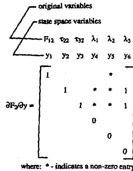
Fig. 10 \partial F_2/\partial y for Two Rigidly Connected, Planar Manipulators on Independent, Vertically Compliant Bases
