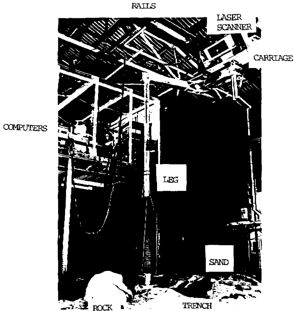
Figure 2: Single leg testbed
