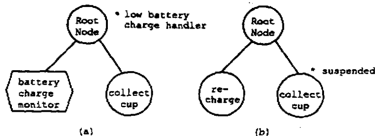
Figure 3-2: Exception handling
