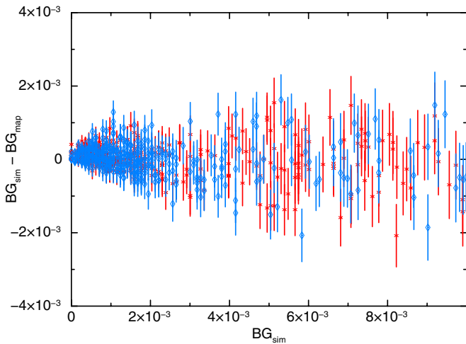
Figure 8. Comparison of the background measured directly from the simulated image ( BG_{\text{sim}} ) with that measured from a background map ( BG_{\text{map}} ) constructed from the simulated image. The red stars show the simulations with no sources included, the blue diamonds the simulations containing a source.
