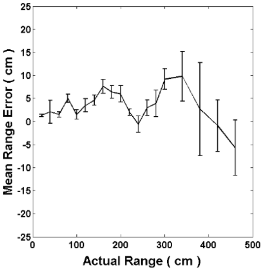
Fig. 8. Close up view of the range accuracy showing the mean of the measured ranges across all bearings: 0^\circ to 90^\circ . The error bars represent the maximum standard deviation. 50 measurements were taken at each position
