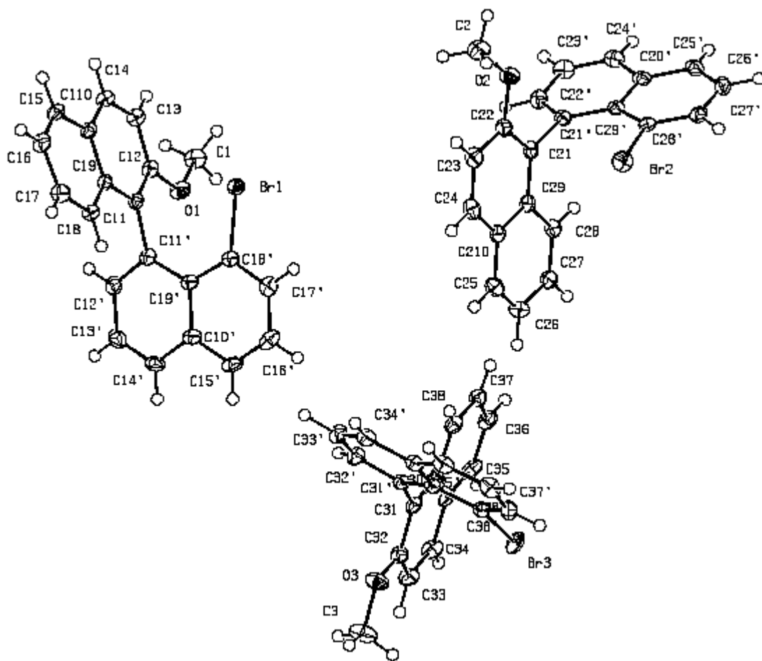
Figure 8. ORTEP diagram of ( \pm )- 18 showing the atom labeling scheme. Displacement parameters are shown at the 50% probability level.
