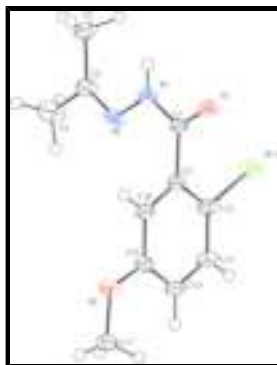
Fig. 1. Perspective view of the title compound with the atom numbering; displacement ellipsoids are at the 50% probability level.
