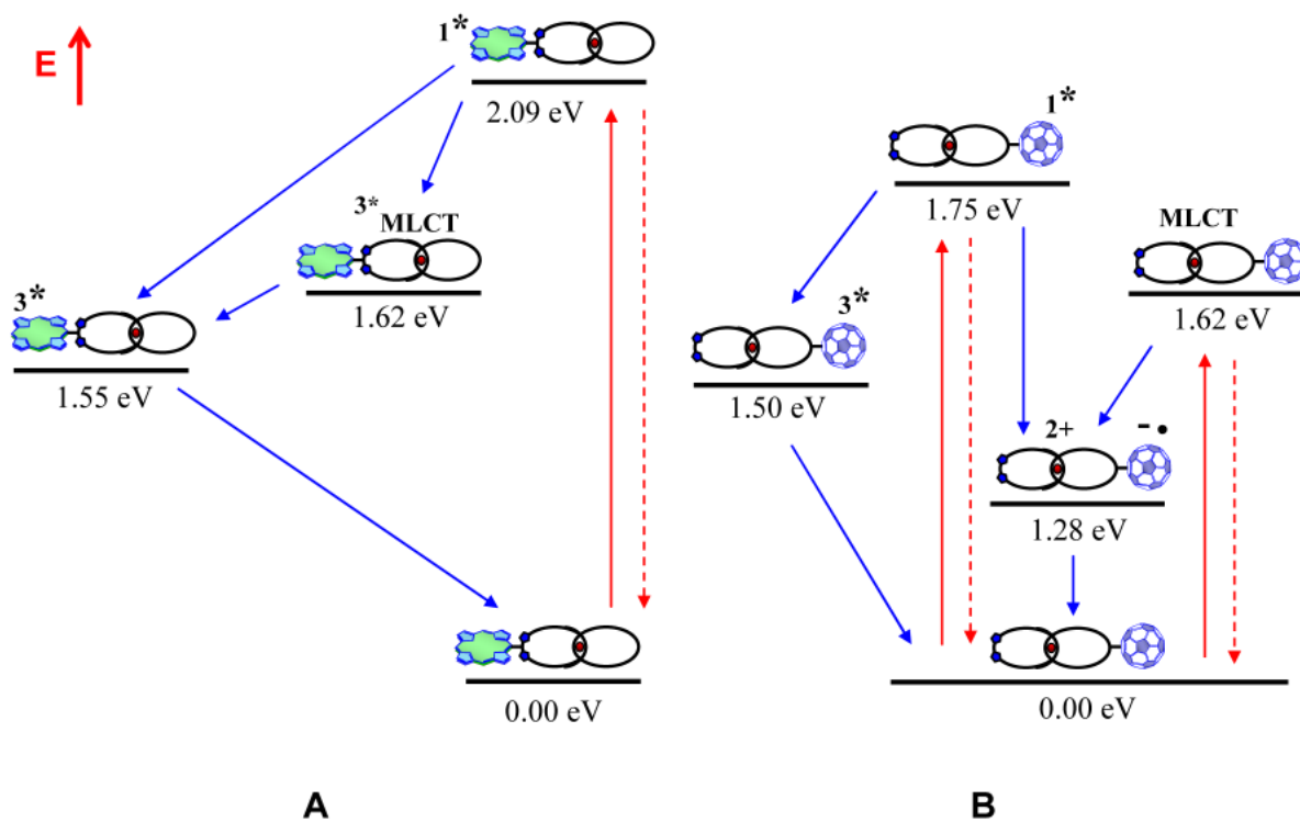
Figure 12. A) Schematic energy level diagrams and decay pathways for catenate 3 upon excitation at 420 nm, and B) catenate 4 upon excitation at 387 or 355 nm.
