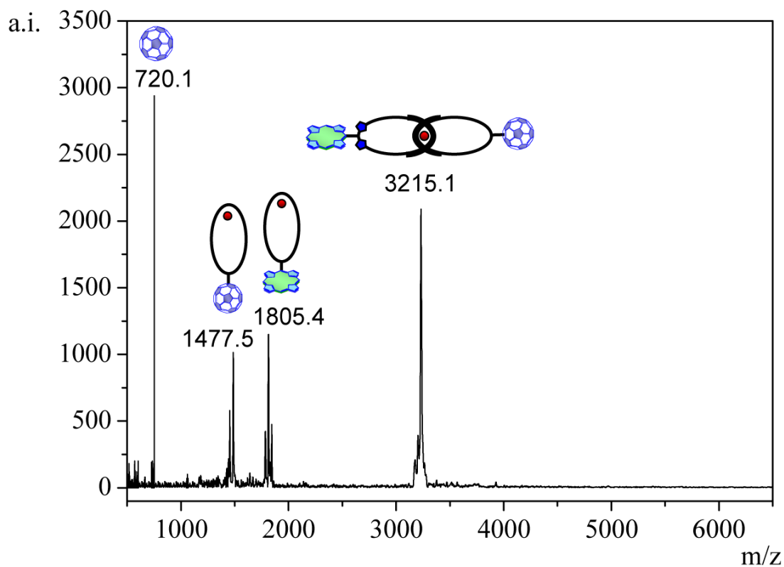
Figure 3. MALDI-TOF mass spectrum of catenate 1 (positive mode, \alpha -cyano-4-hydroxycinnamic acid (CCA) matrix). The absence of peaks between the molecular ion peak and the peaks corresponding to the individual macrocycles is characteristic of catenane structures. 15,21 ● = Cu(I) ion; ● = Zn(II)-porphyrin and ⊕ = C 60 .
