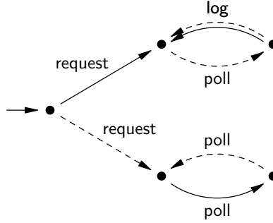
Figure 8: A mixed specification that is not consistent.
