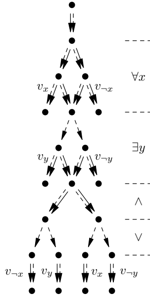
Figure 14: Modal transition system N_{\varphi_Q} representing the evaluation game graph of the formula in (5).
