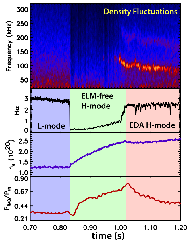
FIG. 26. A sudden transition from the ELMfree to the EDA H-mode is accompanied by a change in impurity confinement and the appearance of the QCM. Greenwald et al. , Fusion Sci. Tech. 51 , 266 (2007). Copyright 2007 American Nuclear Society. 185
