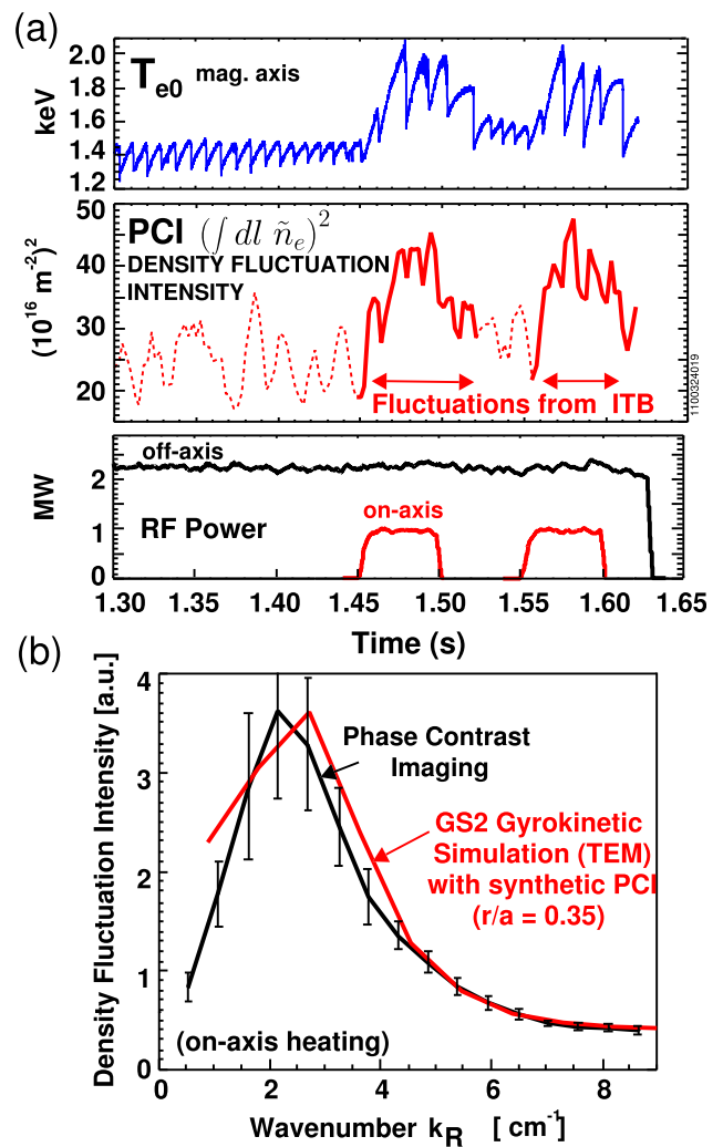
FIG. 50. Modulated on-axis heating in ITB discharges allows measured fluctuations to be localized within the barrier and supports the theory of barrier control via density gradient driven TEMs.
