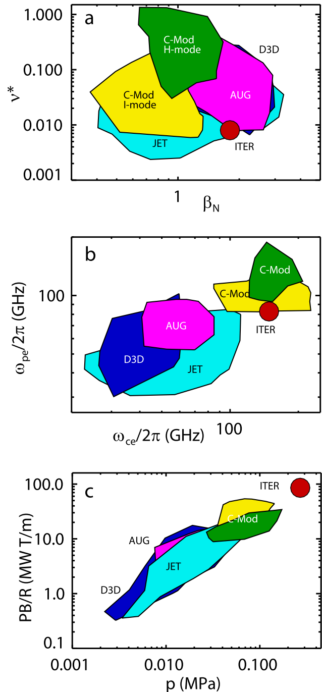
FIG. 1. C-Mod parameters are compared to other tokamaks and those projected for ITER as relevant to physics for (a) core MHD, (b) RF heating and current drive, and (c) boundary plasma physics where PB/R is a proxy for the divertor heat load and the core pressure a proxy for the divertor pressure. Data are mainly from the ITPA H-mode data base and includes C-Mod I-modes for comparison.
