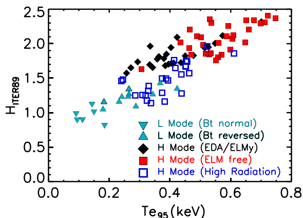
FIG. 37. The energy confinement time, normalized to the ITER89 L-mode scaling law, is plotted vs the pedestal temperature, unifying data over a wide range of parameters and confinement regimes. Reprinted with permission from Greenwald et al. , Nuclear Fusion 37 , 793 (1997). Copyright 1997 IOP. 17
