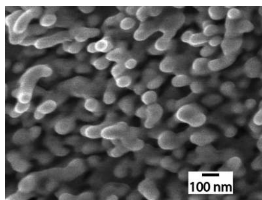
FIG. 6. A micrograph of tungsten nanostructures produced by 13 s of helium discharge time on a target operating at about 2000 K. The morphology and growth rate are essentially identical to what is produced in a linear plasma device under similar conditions. Reprinted with permission from Wright et al. , Nuclear Fusion 52 , 042003 (2012). Copyright 2012 IOP. 51
