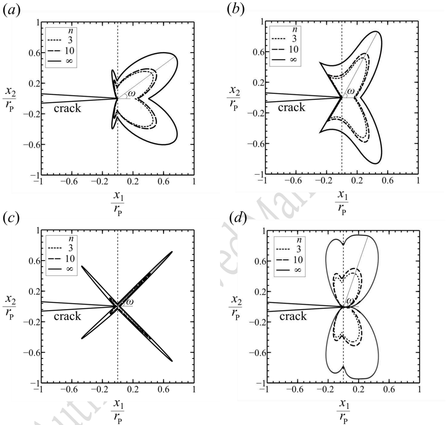
Fig 2. Mode I plastic zone for (a) triangular lattice, (b) kagome lattice, (c) diamond lattice, (d) hexagonal lattice.
