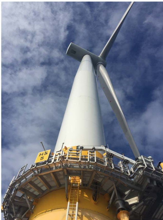
Figure 30. A 6-MW floating wind turbine in Equinor’s 30-MW array near Peterhead, Scotland, supported by a spar buoy floating platform. Photo courtesy of Walt Musial, NREL
