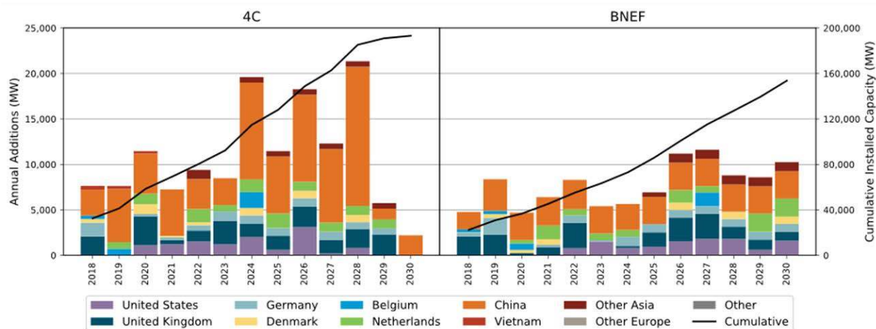
Figure 17. Medium-term wind capacity forecasts by country through 2030
