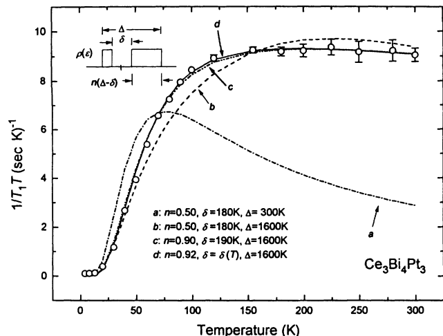
FIG. 12. Fit of 1/T_1T to the model density of states \rho(\epsilon) described by an energy gap of magnitude \delta positioned asymmetrically with respect to the center of the band.
