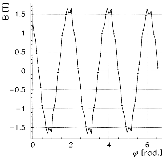
FIG. 7. Azimuthal dependence of B_{rad} for magnet 5 at a radius of 14.9 mm. (The solid line serves to guide the eye.)
