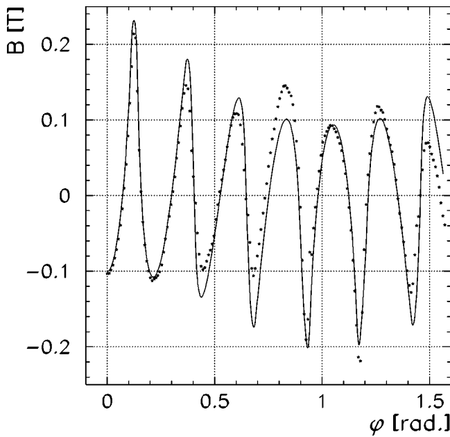
FIG. 9. Multipole components \nu \geq 1 ( \star ), corresponding mainly to a 54 pole ( \nu=1 ), extracted from the measured data shown in Fig. 8 by subtraction of the pure sextupole component \nu=0 from the data. The Halbach series for \nu=1, \dots, 10 of the fit to the data of Fig. 8 with the full series ( \nu=0, \dots, 10 ) is indicated as a solid line.
