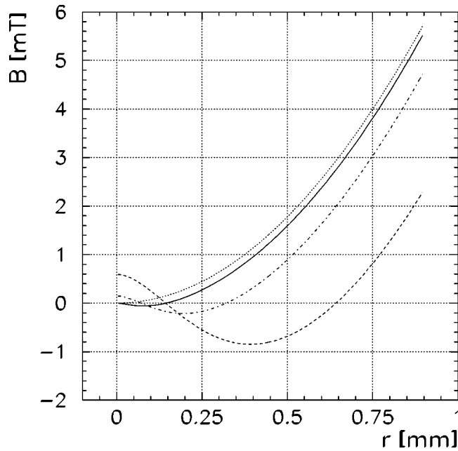
FIG. 15. Radial dependence of the magnetic flux density near the axis of a magnet with B_0=1.6 T and r_1=15 mm for three different Hall probe sizes. The dotted line corresponds to a point-like Hall probe, the solid line to a Hall probe of h=0.2 mm lateral dimension, the dashed-dotted line to h=0.5 mm, and the dashed line to h=1.0 mm.
