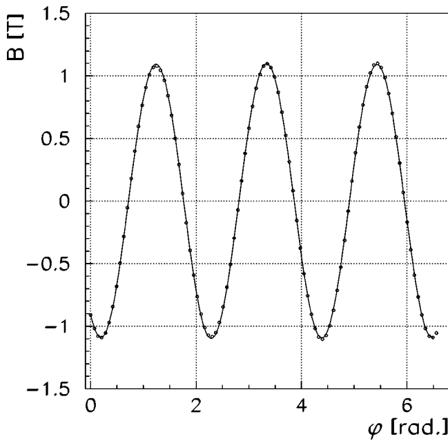
FIG. 6. Azimuthal dependence of B_{rad} for magnet 4 at a radius of 12.5 mm. The solid line represents a fit with a function taking into account the field component normal to the Hall probe and a radial offset [Eqs. (10) and (11)].
