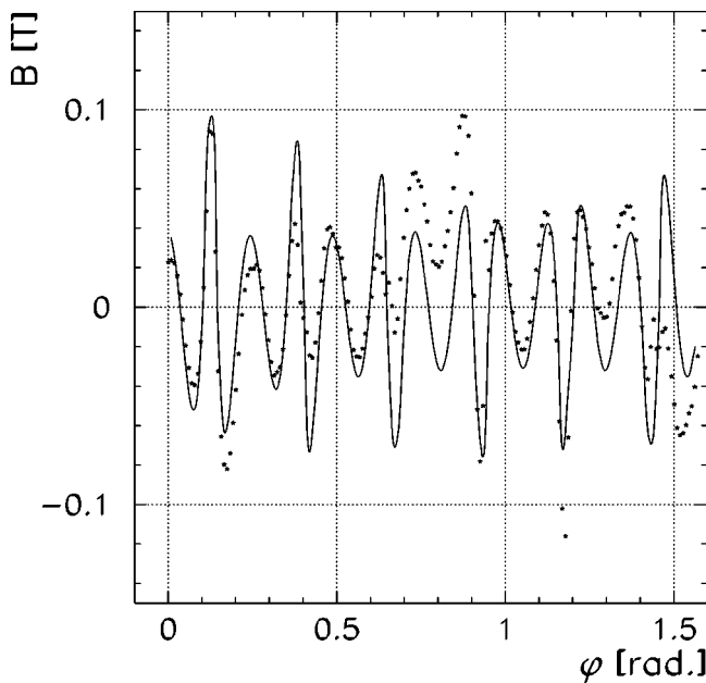
FIG. 10. Multipole components \nu \geq 2 ( \star ) extracted from the data by subtraction of \nu=0 and \nu=1 terms from the data shown in Fig. 8 yield the typical 102-pole structure, corresponding to \nu=2 . Also shown as a solid line is the result of the fit with the Halbach series ( \nu=0, \dots, 10 , shown in Fig. 8) for \nu=2, \dots, 10 only.
