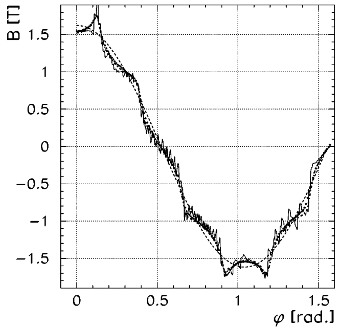
FIG. 8. Azimuthal dependence of B_{rad} for magnet 5 at a radius of 14.9 mm for one quadrant. The measured data ( \star ) are shown together with the results of a MAFIA calculation (thin solid line). A fit to the data with Eqs. (10) and (11) for \nu=0, \dots, 10 of the Halbach series using as a free parameter an average remanence J is indicated (dash-dotted) and yields J=1.293\pm 0.008 T, in good agreement with the expectation J^{yp}=1.283 T. The multipole amplitudes in the fit were corrected as described in Appendix A, in order to account for the finite size of the Hall probe. The \nu=0 term of that fit alone (pure sextupole) is indicated as well (dashed line).
