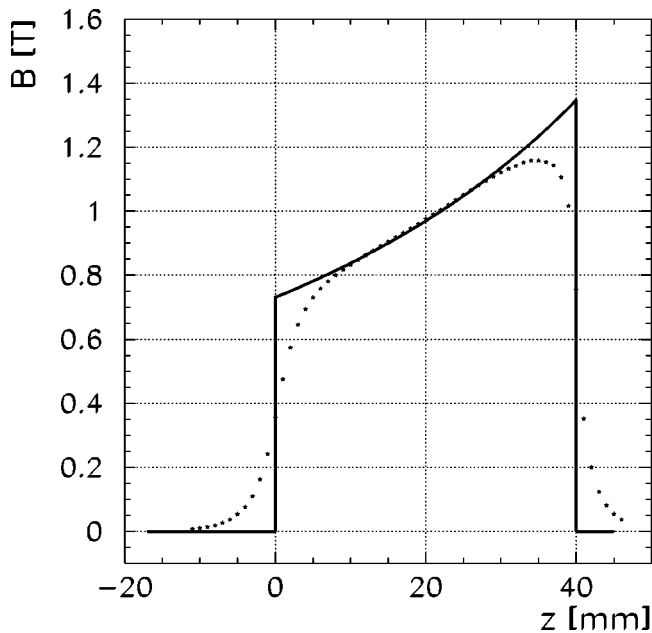
FIG. 12. Measured magnetic flux density B_{\text{rad}} along the axis of magnet 1 ( \star ) at a radius of 4.5 mm at \phi=0 . The solid line corresponds to the result of a calculation based on the measured pole-tip field B_0^* (Table III), using a factor (r/r_1)^2 \cdot [1 - (r_1/r_2)^2] to account for the radius r at which the distribution was measured and for the change in material thickness.
