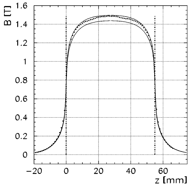
FIG. 11. Magnetic flux density B_{\text{rad}} ( \star ) along the axis of magnet 6 at a radius of 14.5 mm at \phi=0 . The upper solid line indicates the result of a MAFIA calculation using typical values for the remanence J^{\text{yp}} of the individual segments (Table I). The lower solid line for the configuration with minimal values of the magnetization is obtained by scaling the results obtained with J^{\text{yp}} by a factor J^{\text{min}}/J^{\text{yp}} . The dashed lines correspond to the physical boundaries of the magnet.
