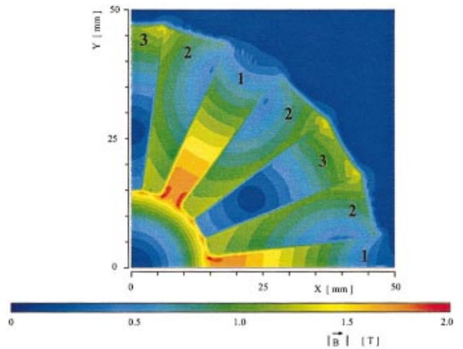
FIG. 2. (Color) Magnitude of the magnetic flux density |\vec{B}| in the central xy plane of sextupole magnet 5 (see Table II for dimensions), calculated using MAFlA. The number code reflects the employed material properties listed in Table I. The original direction of magnetization in the material prior to assembling is indicated in Fig. 1.
