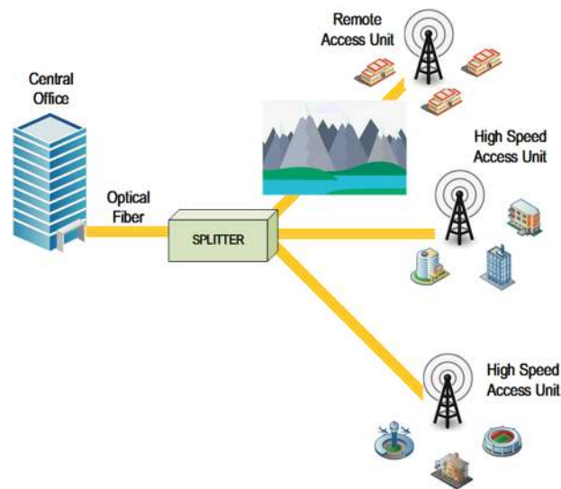
FIG. 2. Structure and application scenarios of RoF systems.
