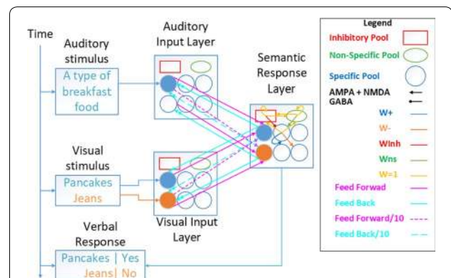
Fig. 1 Implementation of the semantic category judgement task in the model
