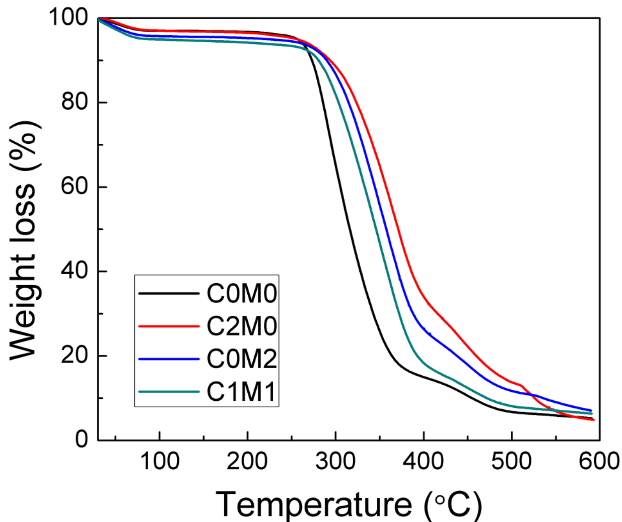
Fig 5. TGA of PVA electrospun nanofibers containing CNC and Ti_3C_2T_x fillers.
