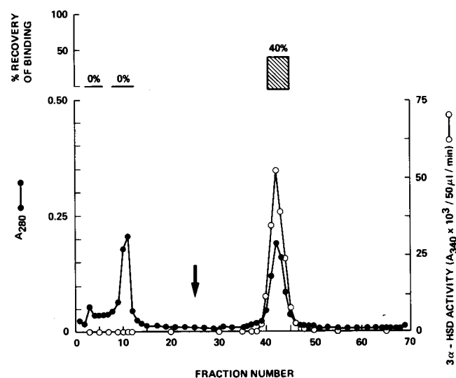
Figure 3. Affinity chromatography of 3 \alpha -hydroxysteroid dehydrogenase-I on PAP-agarose. 35 ml of pooled 3 \alpha -hydroxysteroid dehydrogenase-I from chromatofocusing was applied to a 1 \times 10-cm column of PAP-agarose and eluted with a linear salt gradient (see Methods for detail). Arrow identifies the initiation of the salt gradient. Fractions (2.9 ml) were assayed for protein absorbance (solid circle) and 3 \alpha -hydroxysteroid dehydrogenase activity (open circle) as in Fig. 1. Pooled protein peaks were assayed for lithocholic acid binding and results are expressed as percent of total binding activity applied to the column (upper panel).
