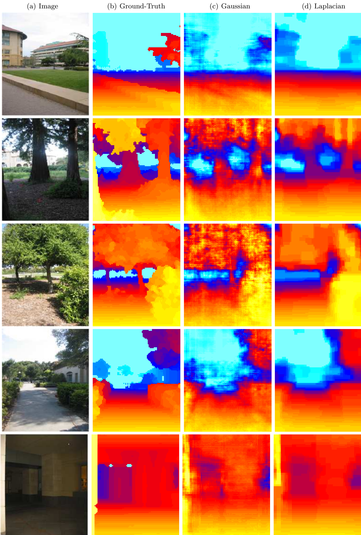
Figure 6: Results for a varied set of environments, showing (a) original image, (b) ground truth depthmap, (c) predicted depthmap by Gaussian model, (d) predicted depthmap by Laplacian model. (Best viewed in color).
