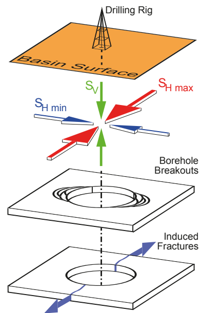
Figure 10. General assumption of stresses in sedimentary basins: the vertical stress ( S_V ) is a principal stress, thus perpendicular to the minimum and maximum horizontal stress ( S_{Hmin} and S_{Hmax} ). Borehole breakouts occur in orientation of the S_{Hmin} , and induced tensile fractures occur in orientation of S_{Hmax} .
