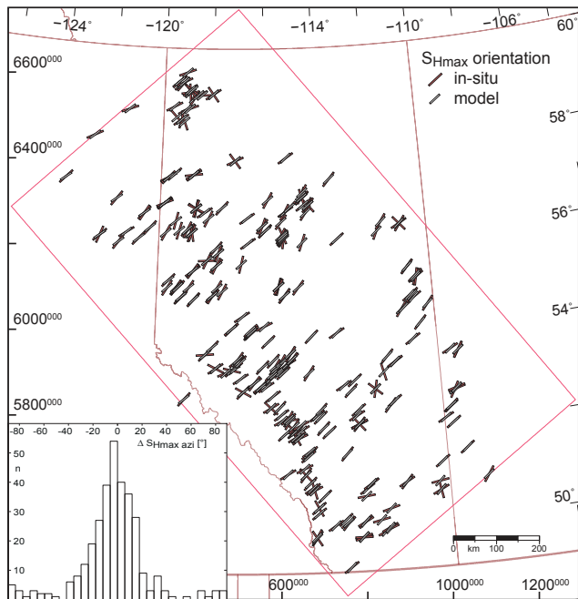
Figure 17. Spatial distribution of the modelled and in situ S_{Hmax} azimuth data. A good fit of the modelled data is reached, except for some suggested misinterpreted data (around \pm 90^\circ ) and systematic rotations close to the Peace River Arch ( 56^\circ N, 118^\circ W) and close to the Bow Island Arch ( 50^\circ N, 114^\circ W). The map extent is indicated by geographical coordinates (top and right) and by UTM coordinates from zone 11 (left and bottom).
