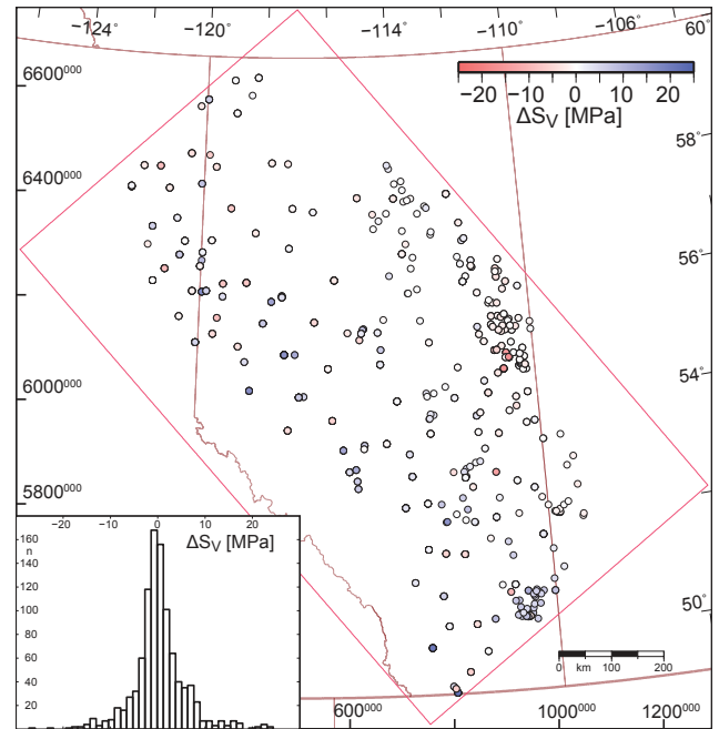
Figure 16. Spatial distribution of \Delta S_V differences are plotted colour coded. The map extent is indicated by geographical coordinates (top and right) and by UTM coordinates from zone 11 (left and bottom).
