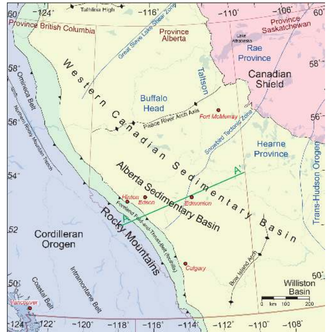
Figure 2. Tectonic map of Alberta and surroundings displaying the important structural features. Blue lines and labels indicate Precambrian structures in the basement. Provincial boundaries and areas are indicated by reddish-brown colours, and tectonic features are labelled in black. The trace of the cross section in Fig. 3 is indicated by a green line. The map is modified and redrawn after Wright et al. (1994).
