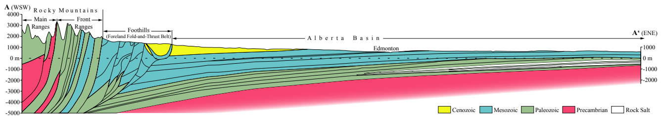
Figure 3. Cross section across Alberta in west–southwest to east–northeast orientation; the trace is highlighted in Figs. 2 and 4. Visible is the Alberta Basin as a wedge-shaped retro-arc foreland basin, together with parts of the Rocky Mountains and the foreland fold-and-thrust belt (foothills) in between. The rock units are roughly indicated by the stratigraphic age. Additional thick rock salt units are indicated separately, because of their potential to detach the stress field. The vertical exaggeration is 10 times, redrawn after Hamilton et al. (1999).
