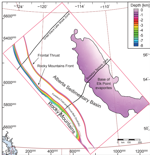
Figure 7. Upper crustal structures used in the model. The units above the basement are separated in the basin, the foothills and the Rocky Mountains. The basin also contains a thin rock salt layer from the Elk Point group. Within the basement, the Great Slave Lake Shear Zone and the Snowbird Tectonic Zone are incorporated. The map extent is indicated by geographical coordinates (top and right) and by UTM coordinates from zone 11 (left and bottom).
