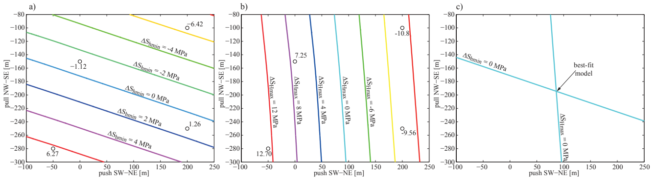
Figure 15. Plot of four models with different shortening or extension at the model boundary; see Table 2 for details. (a) and (b) : the median S_{hmin} and the median S_{Hmax} are plotted depending on the northwest to southeast extension (pull) and the southwest to northeast shortening (push). The isolines of the median \Delta S_{hmin} and \Delta S_{Hmax} are colour coded. (c) The isolines where the median \Delta S_{hmin} and \Delta S_{Hmax} are zero are plotted alone. The intersection of both isolines indicated the push-pull values where the best-fit model can be found.
