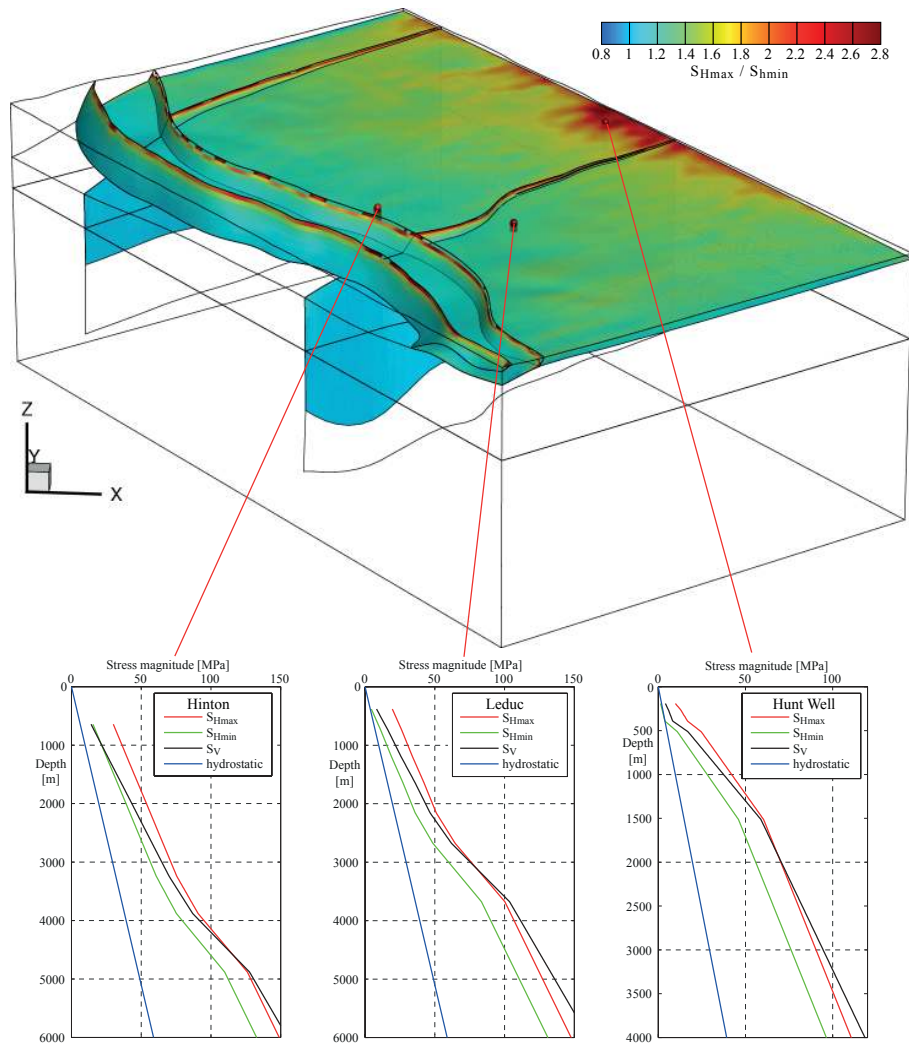
Figure 20. 3-D view of the best-fit model. Displayed is the S_{Hmax}/S_{Hmin} ratio, plotted at the basement top, along the Snowbird and Great Slave Tectonic Shear Zone, the Rocky Mountains front and the front of the foothills. Three virtual wells from the surface down into the basement are indicated in the model. The stress growth into depth is illustrated in the lower part. These are virtual wells in Hinton, in Leduc (30 km south of Edmonton) and the location of the Hunt well (15 km west of Fort McMurray). The shallowest part is not shown in the plots due to free surface effects.
