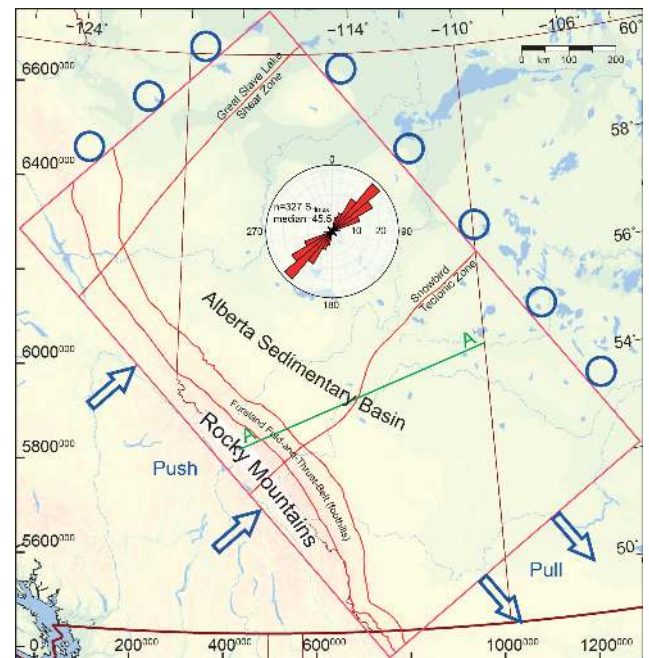
Figure 4. Map of Alberta with the model extent (red box) combined with the model features. Implemented are the main structural features (red lines), which are the front of the Rocky Mountains and the foothills, respectively, as well as the Snowbird Tectonic Zone and the Great Slave Lake Shear Zone. For comparison, see the tectonic map (Fig. 2). Push and pull along model sides and the allowed lateral motion are indicated by blue arrows and circles, respectively. The mean orientation of S_{Hmax} is indicated by a rose diagram; note that stress orientation is parallel and orthogonal, respectively, to the model box. The trace of the cross section in Fig. 3 is indicated by the green line.
