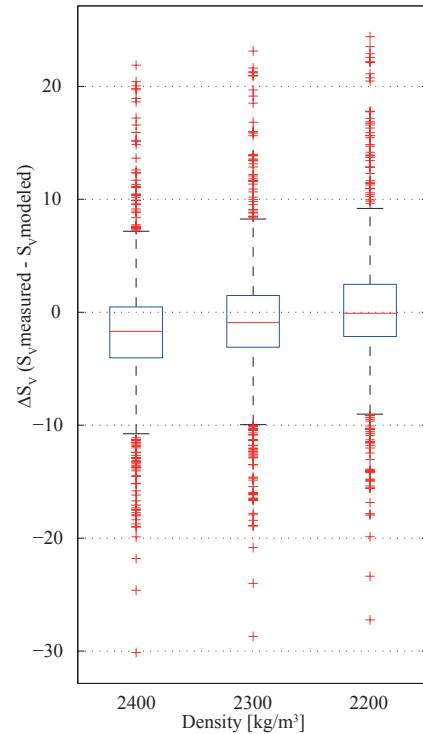
Figure 13. Boxplot of the varied density of the basin sediments – plotted is the \Delta S_V . The median \Delta S_V of the model with a density of 2200 \text{kg m}^{-3} is close to 0 MPa and therefore the best-fit density to the available S_V data, in contrast to the models with a higher basin density, where \Delta S_V is negative (see Eq. 11).
