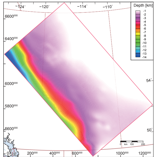
Figure 6. Topography of the basement top is shown within the model box. The map extent is indicated by geographical coordinates (top and right) and by UTM coordinates from zone 11 (left and bottom).
