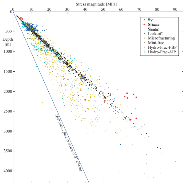
Figure 12. Depth plot of the in situ stress magnitudes. These are 981 S_V magnitude data (black), 1720 S_{hmin} magnitudes (several colours), and 2 measured as well as 11 calculated S_{Hmax} magnitudes (highlighted red points). S_{hmin} data are colour coded depending on the test type, which is taken over from the original database.
