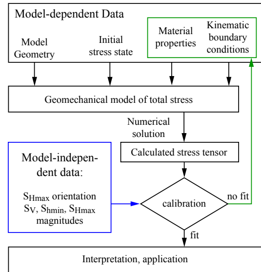
Figure 1. Sketch of the general workflow. The geomechanical model is prepared based on the model geometry, the material properties, the variable displacement boundary conditions and the initial stress state. The numerically modelled total stress tensor is calibrated on model-independent in situ stress data until the model fits the calibration data.
