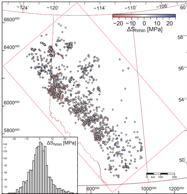
Figure 18. Comparison of the modelled and in situ S_{hmin} magnitudes, plotted as \Delta S_{hmin} . The map extent is indicated by geographical coordinates (top and right) and by UTM coordinates from zone 11 (left and bottom).
