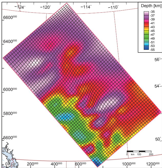
Figure 5. Topography of the Mohorovičić discontinuity (Moho) within the model box. The map extent is indicated by geographical coordinates (top and right) and by UTM coordinates from zone 11 (left and bottom). The mesh size ( \sim 20 km) at that depth is indicated by black lines.
