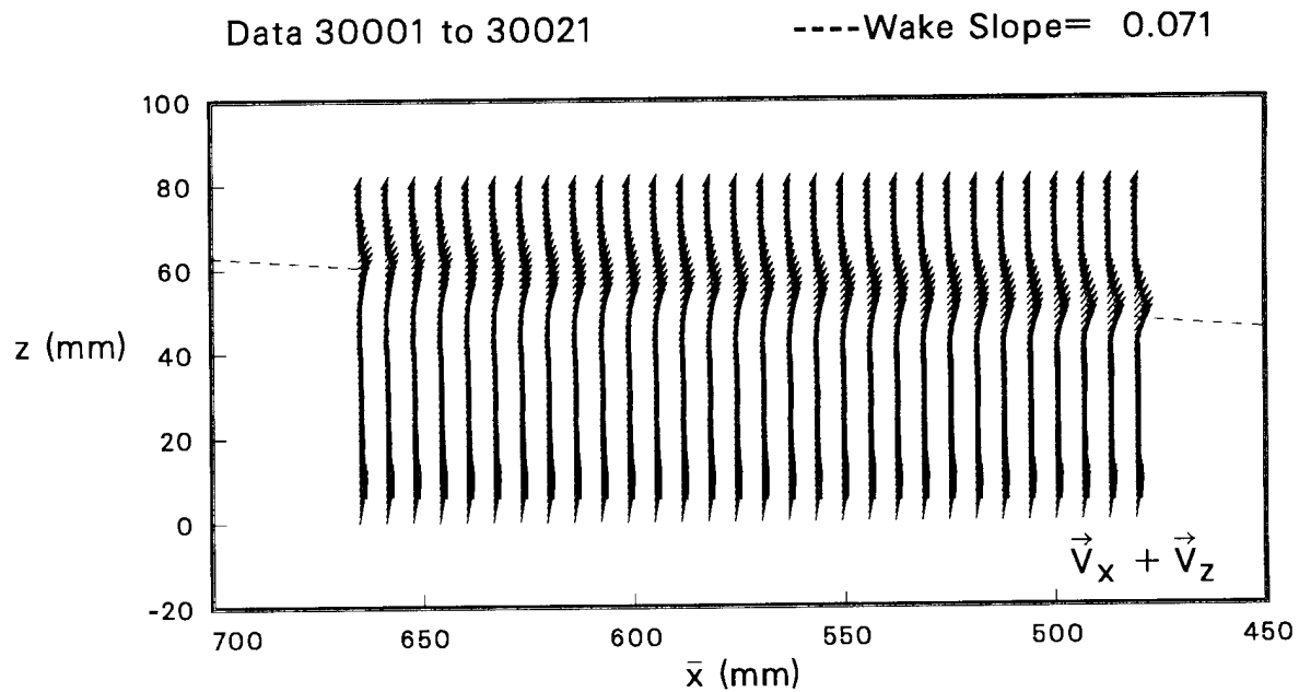
Figure 45. Velocity-vector field in the x - z plane passing through y = 40 mm during the time that the tip of the rotor blade advanced from 2.5 to 3.5 chord lengths. The rotor speed was 1100 rpm.
