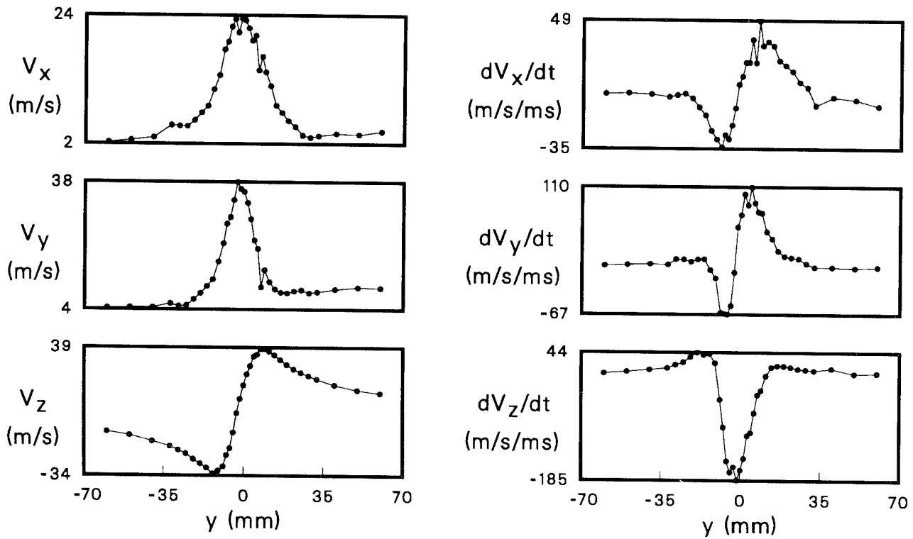
Figure 19. Velocity components along a horizontal sweep across the trailing vortex after the blade tip moved forward 3 chord lengths. The rotor speed was 1100 rpm.
