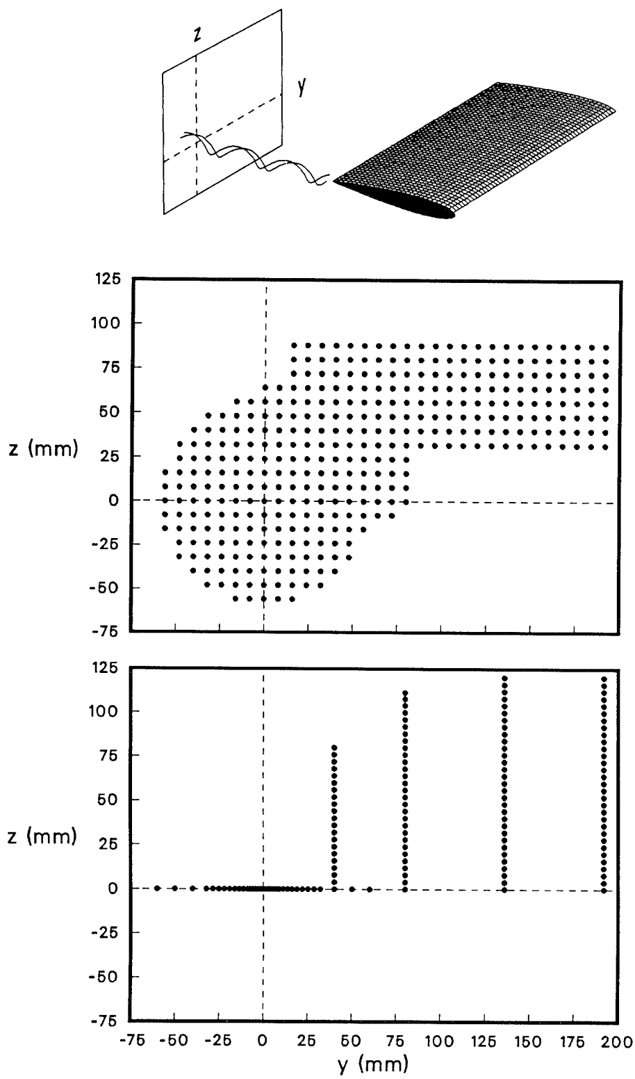
Figure 15. Measurement locations over the y - z plane in the wake of the rotor blade. The approximate center of the trailing vortex defines the (0,0) position.
