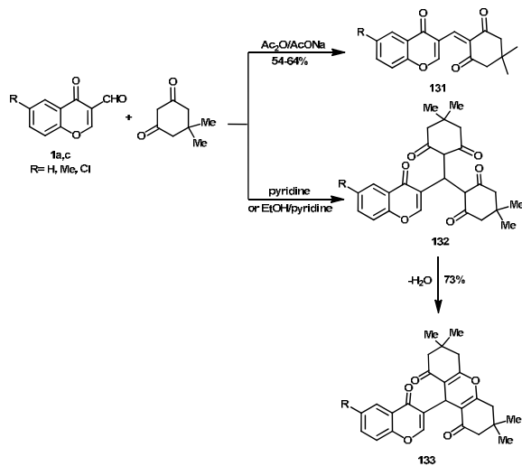
Scheme 63
