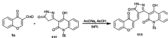
Scheme 54
