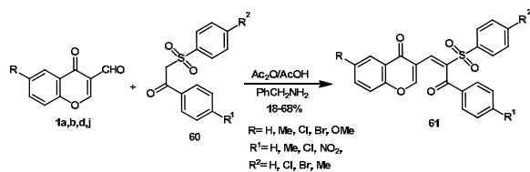
Scheme 28
