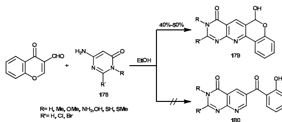
Scheme 87
