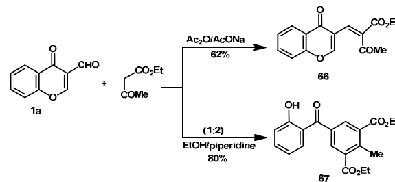
Scheme 31
