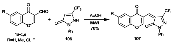
Scheme 52
