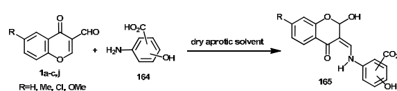
Scheme 80
