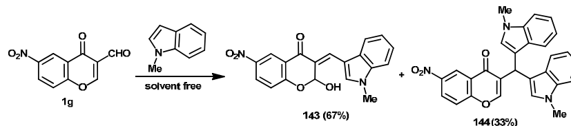
Scheme 69
