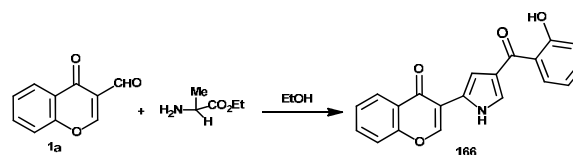
Scheme 81
