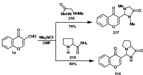
Scheme 101
