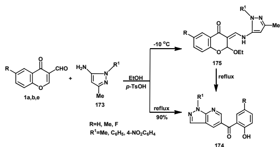
Scheme 85
