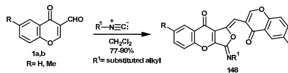
Scheme 72
