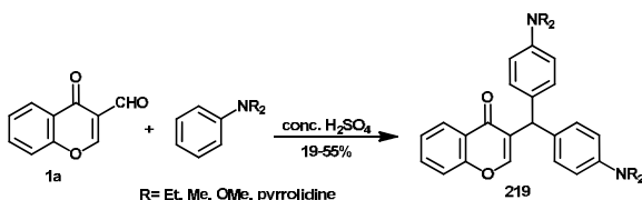
Scheme 102
