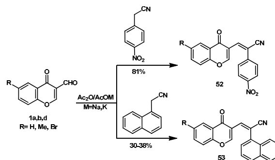
Scheme 24
