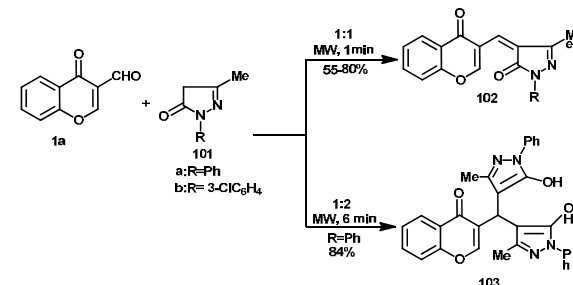
Scheme 50
