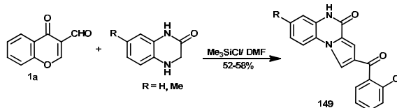
Scheme 73
