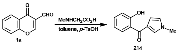
Scheme 100
