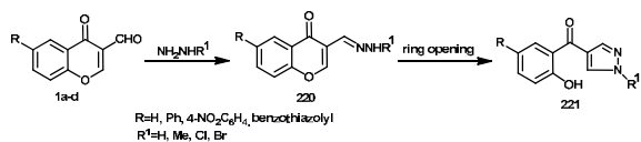
Scheme 103
