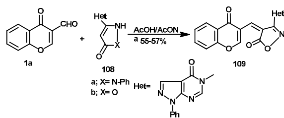
Scheme 53
