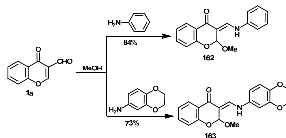
Scheme 79
