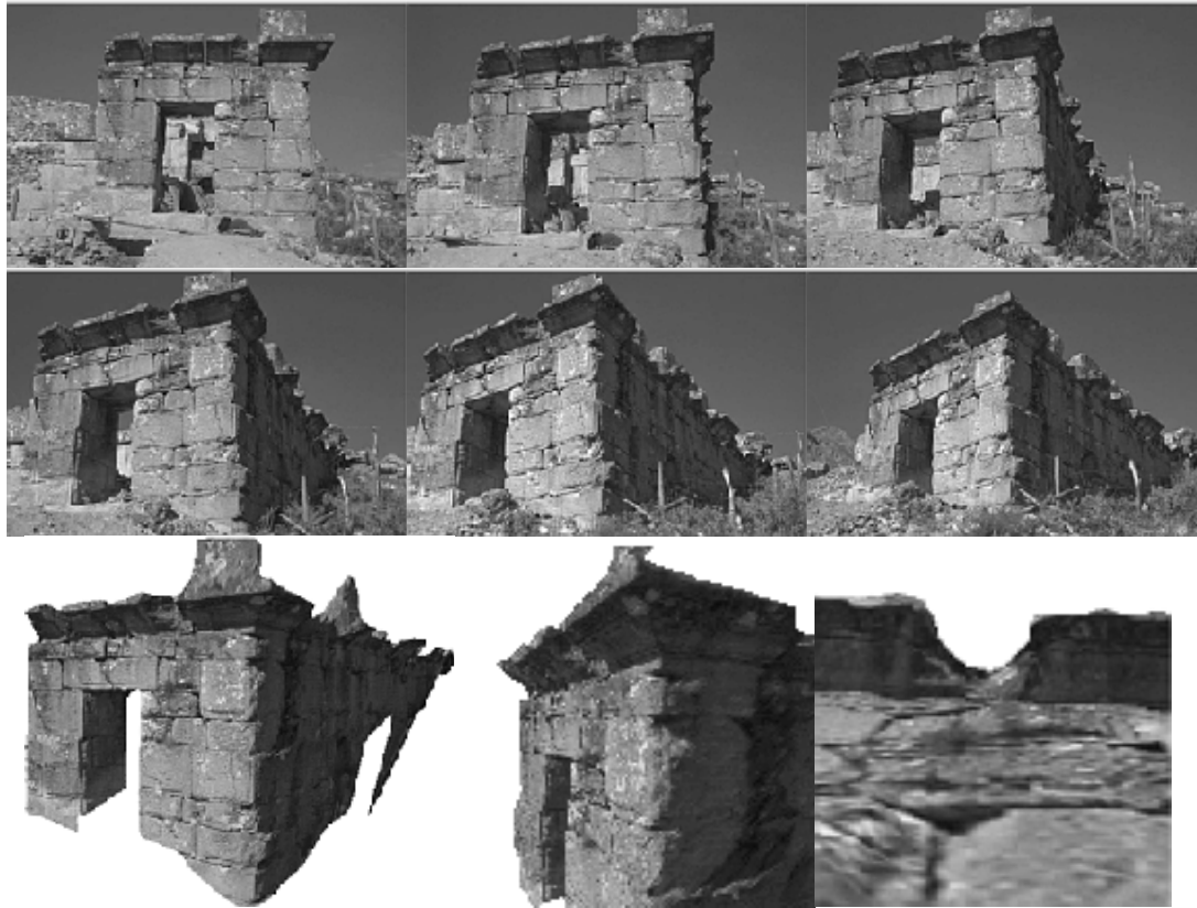
Figure 2 Corner of the Roman baths at Sagalassos. Top: 6 photographs used for modelling, Bottom: different views of the 3D reconstruction.
