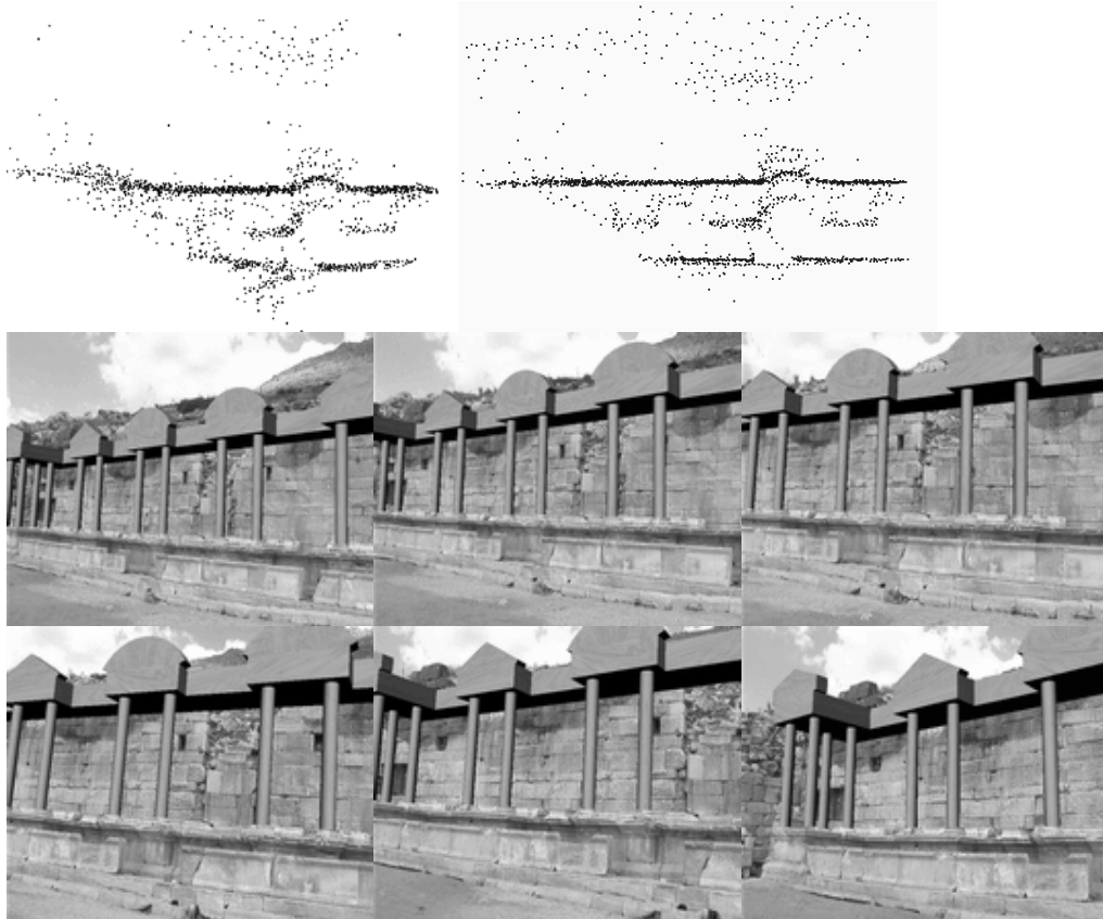
Figure 8 Fusion of real and virtual fountain parts. Top: Structure before and after bundle adjustment. Bottom: 6 of the 250 frames of the fused video sequence.
