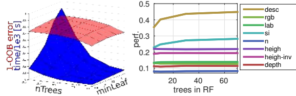
Figure 3. Parameters of the 3D classifier. Left: performance (red) and test time (blue) w.r.t. the number of trees and the minimum number of observations per leaf. Right: the performance of each descriptor part individually (and the final descriptor-desc) using RF classifier.
