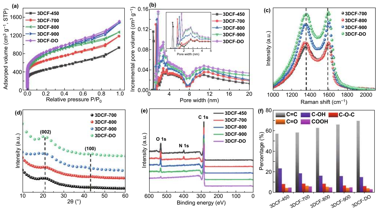
Fig. 2 a N_2 adsorption and desorption isotherms, b corresponding pore size distributions, c Raman spectra, d powder XRD patterns, e survey spectra and f 1s deconvoluted spectra of 3DCF materials
