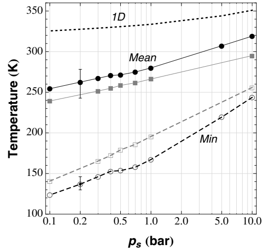
Fig. 2. Globally averaged (solid, filled) and minimum (dashed, empty) temperatures as a function of surface pressure for Gl 581 c (black circles) and HD 85512 b (gray squares). For comparison, the surface temperature of the 1D model for Gl 581 c is also shown (dotted curve). The error bars on the 200 mbar case show the temperatures reached by varying the surface albedo between 0.1 and 0.5.
