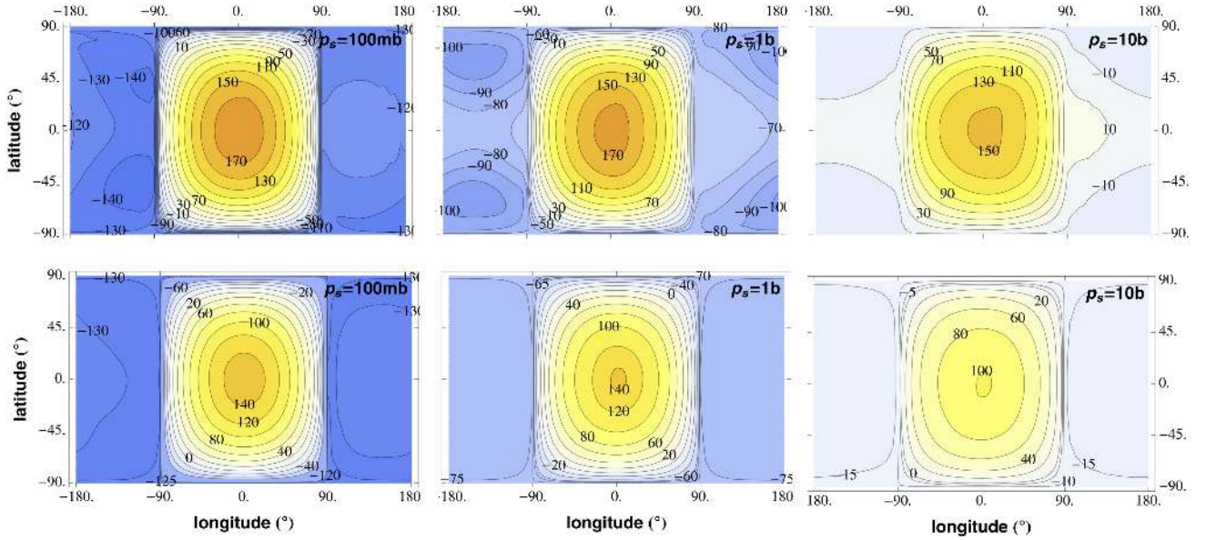
Fig. 1. Surface temperature maps (in °C) for the dry Gl 581 c ( top row ) and HD 85512 b ( bottom row ) runs for a total pressure ( p_s ) of 0.1, 1 and 10 bars ( from left to right ). Longitude 0° corresponds to substellar point.
