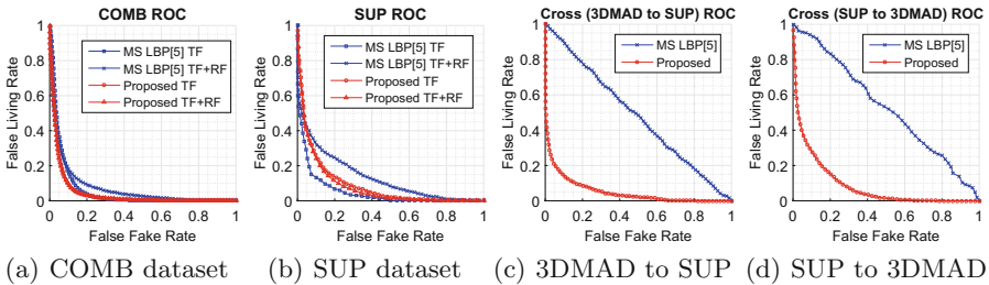
Fig. 4. ROC curves under intra-database and cross-dataset protocol. Note that the legend TF and RF means Thatsmyface mask and REAL-F mask.
