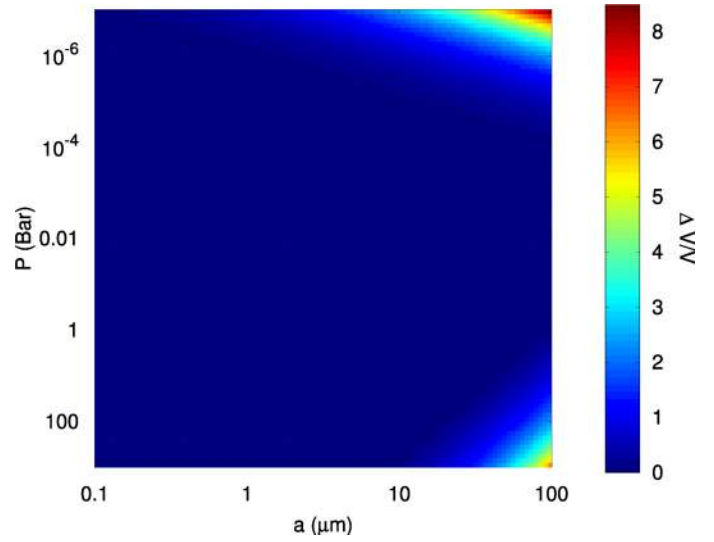
Fig. A.1. Ratio of the Cunningham velocity to the more sophisticated model of the particle settling velocity considered in the Appendix.
