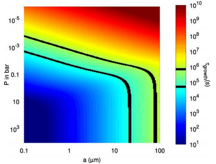
Fig. 15. Approximate growth time scale of \text{TiO}_2 grains in HD 209458b. The bottom black line shows the advective timescale and the top one is ten times the advective timescale.
