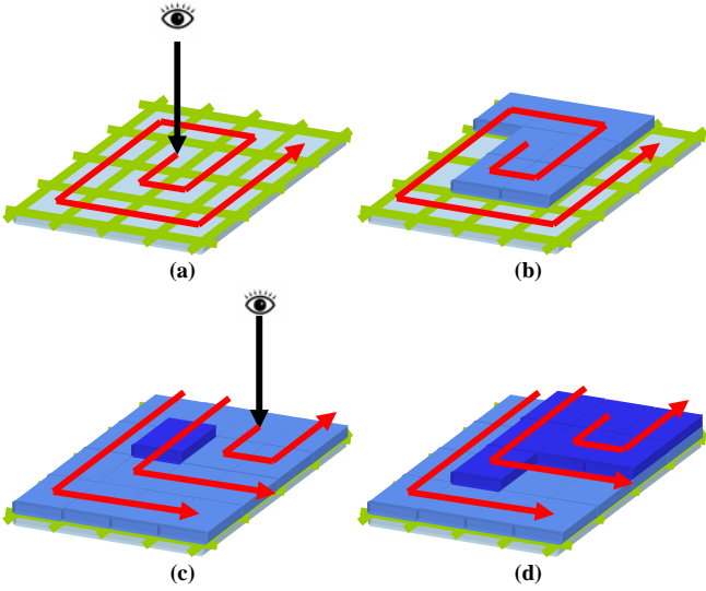
Fig. 5. (a) Given the image with lowest resolution, we find a block which contains the user's viewing pixel and decide the sequence of the following blocks. (b) After the blocks at the lowest level have been transmitted, the blocks at the next level will be transmitted as the same sequence. (c) & (d) If the user changes the viewpoint, the sequence will be recomputed.
