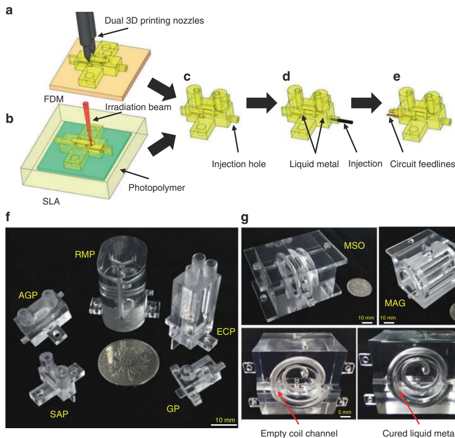
Fig. 1 3D printing and manufacturing procedure of integrative MR probeheads for different scenarios. Both a fused deposition modeling (FDM) and b stereo lithography appearance (SLA) techniques are utilized to fabricate a complete probehead (c) layer by layer according to the simulation design. d Liquid metal is perfused into the model through the injection hole to form an RF coil. e The RF coil is connected to the matching circuit by two copper strips to form a complete probe. The entrance and exit of the liquid metal channel are completely sealed with silver paste. Various 3D-printed probeheads suitable for MR applications can be fabricated and utilized, including f U-tube saddle probehead (SAP), U-tube Alderman-Grant probehead (AGP), reaction monitoring probehead (RMP), electrochemical reaction monitoring probehead (ECP), gradient probehead (GP) for MR, and g modified solenoid imaging probehead (MSO), modified Alderman-Grant imaging probehead (MAG) for MRI. The coil channel of MSO probehead, before and after the liquid metal perfusion, are also shown.
