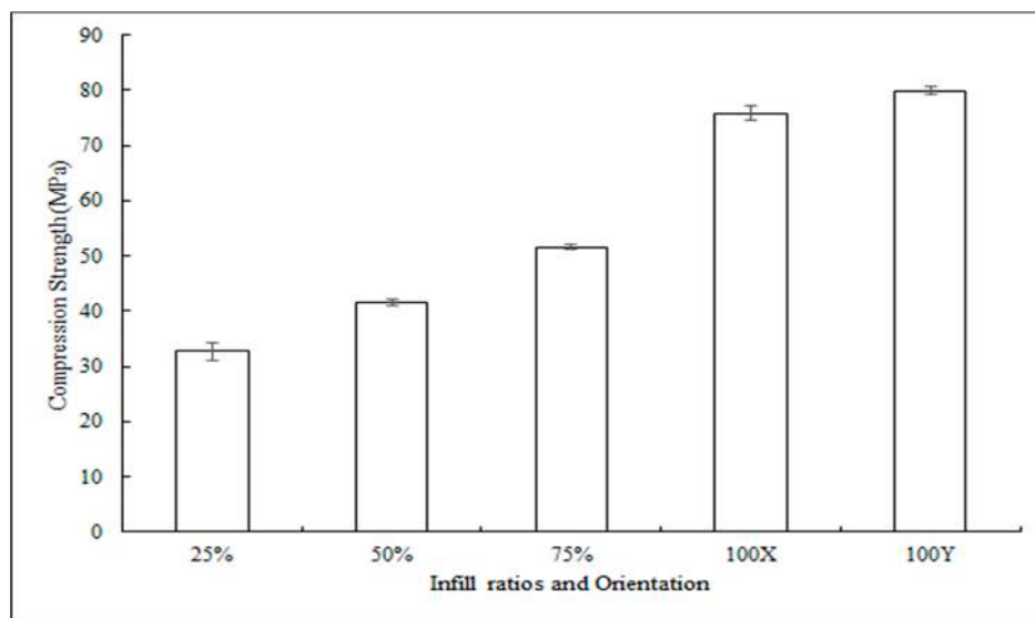
Figure 8. Compressive strengths of samples printed with different infill ratios and in various orientation constructs (mean \pm SD, n = 5). * for p < 0.05.
