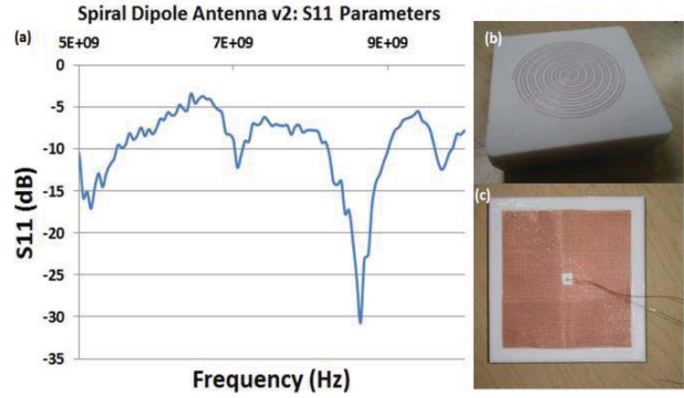
Fig. 6. Experimental S11 parameters of a dipole antenna with an embedded/encapsulated mesh back reflecting plane (a). The spiral antenna after embedding (b), and the back reflecting plane before embedding and encapsulation (c).
