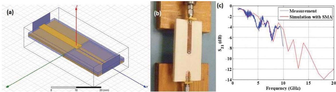
Fig. 8. A multilayer micro-strip designed in HFSS (a). The micro-strip being tested for S_{21} (b), this was after construction was completed and two SMA connectors were soldered to the mesh micro-strip. Measured and simulated S_{21} results are shown in (c), the micro-strip appears high loss due to impedance miss-match at the SMA connector.
