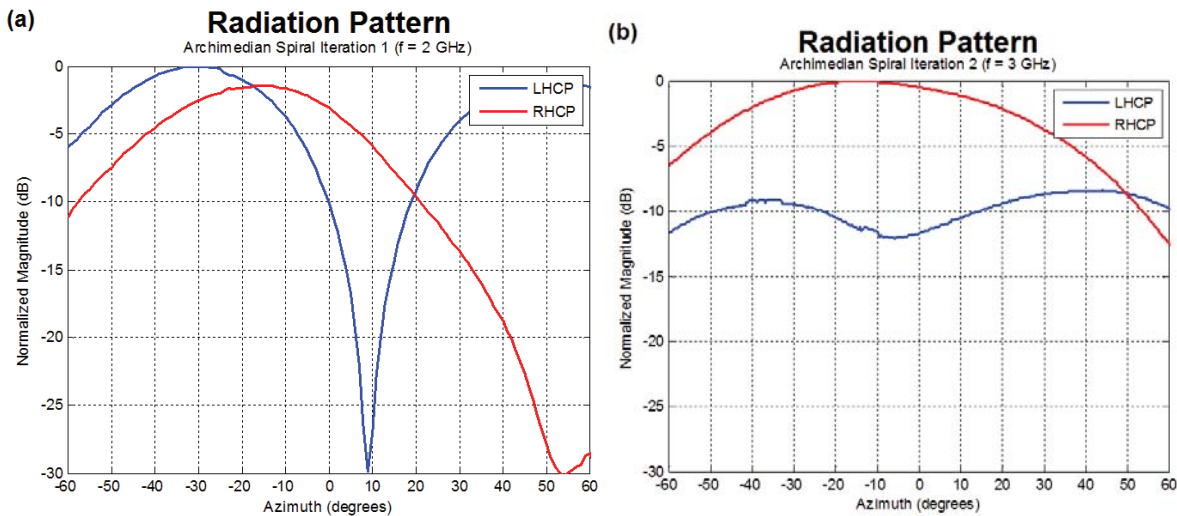
Fig. 5. Experimental and simulated (a) radiation pattern Archimedian spiral antenna v1 at a frequency of 2.0 GHz. The (b) radiation pattern of the Archimedian spiral with an embedded back reflecting plane is shown at a frequency of 3.0 GHz.
