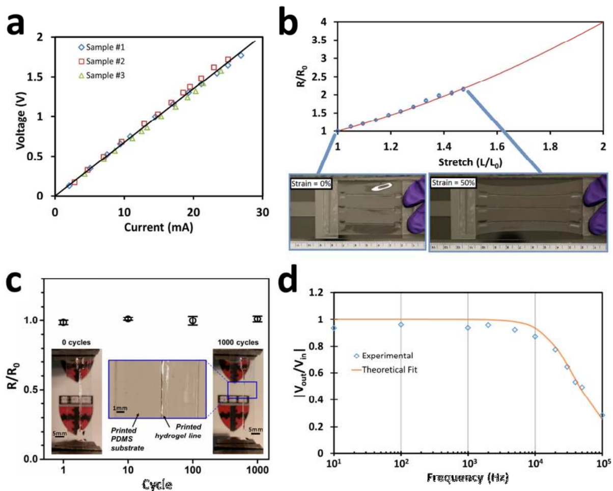
Figure 4. Electrical characterizations of the hydrogel in either bulk or printed state. a) I-V curves obtained from 4-point probe measurements performed on bulk hydrogel samples. Sample dimensions were on average 30 cm long, 4.2 mm wide, and 3.5 mm in height, with an average measured resistance of 67.3 \pm 2.4 \Omega ; this corresponds to a conductivity of 10.39 \pm 0.31 \text{ S m}^{-1} . b) The normalized resistance of printed hydrogels on a PDMS substrate is measured as a function of stretch, plotted against the ideal geometric behavior. Photos illustrate the sample in the initial (strain = 0%) state and the fully stretched (strain = 50%) state with the mechanical load applied only to the PDMS. c) The normalized resistance of printed hydrogels on a PDMS substrate as a function of fatigue cycle number. Uniaxial tensile strain cycles of 20% strain were performed for up to 1000 cycles. No significant change to the resistance vs. strain behavior was observed during our tests. Comparing images both before and after fatigue tests illustrate the lack of visible damage or delamination d) The transfer function of an ionic cable design is plotted against frequency. We perform a theoretical fitting of our results using a simple RC circuit model for the ionic cable and can observe a reasonable level of agreement between experimental results and theory.
